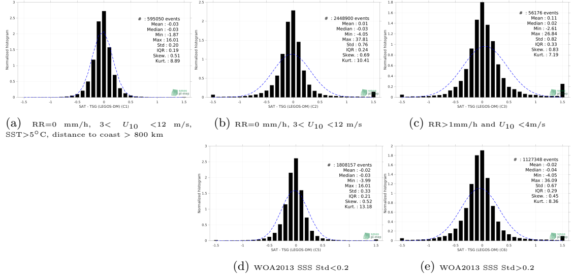
Figure 13: Normalized histogram of \Delta SSS (SMOS SSS L4 v1 - Monthly (CMEMS-CNR) - TSG (LEGOS-DM)) for 5 different subdatasets corresponding to: RR=0 mm/h, 3 < U_{10} < 12 m/s, SST>5°C, distance to coast > 800 km (a), RR=0 mm/h, 3 < U_{10} < 12 m/s (b), RR>1mm/h and U_{10} < 4 m/s (c), WOA2013 SSS Std<0.2 (d), WOA2013 SSS Std>0.2 (e).
