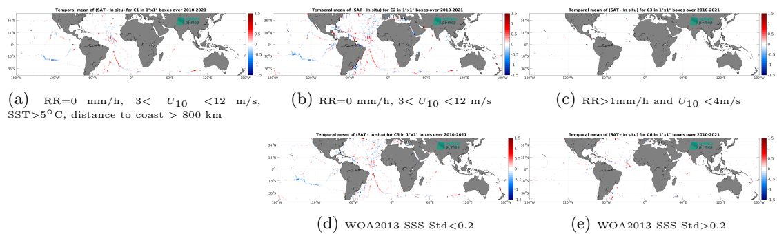
Figure 14: Temporal mean gridded over spatial boxes of size 1^\circ \times 1^\circ of \Delta\text{SSS} (SMOS SSS L4 v1 - Monthly (CMEMS-CNR) - TSG (GOSUD-Sailing-ship)) for 5 different subdatasets corresponding to: RR=0 mm/h, 3 < U_{10} < 12 m/s, SST > 5°C, distance to coast > 800 km (a), RR=0 mm/h, 3 < U_{10} < 12 m/s (b), RR > 1mm/h and U_{10} < 4 m/s (c), WOA2013 SSS Std < 0.2 (d), WOA2013 SSS Std > 0.2 (e).
