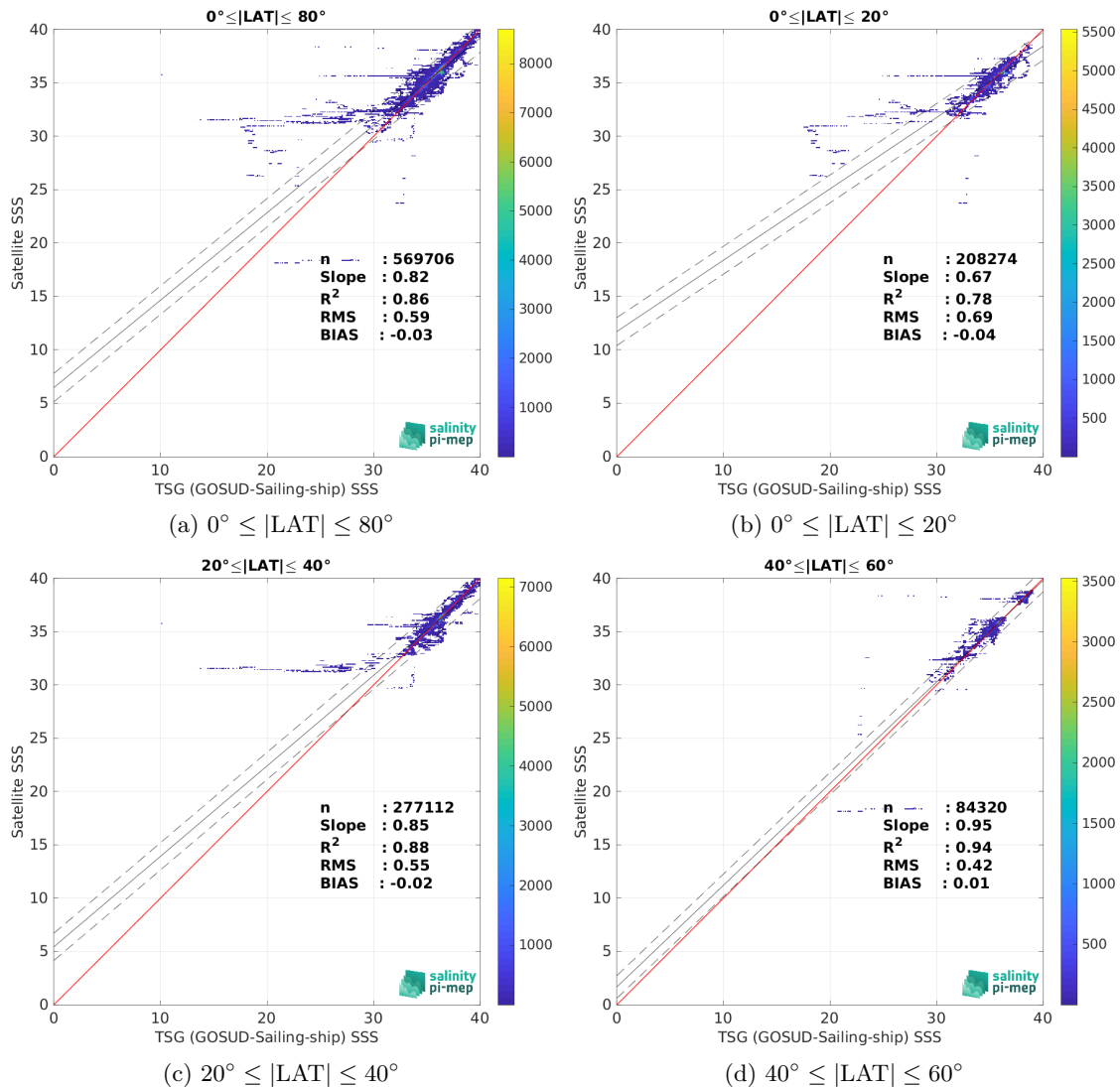
Figure 10: Contour maps of the concentration of SMOS SSS L4 v1 - Monthly (CMEMS-CNR) SSS (y-axis) versus TSG (GOSUD-Sailing-ship) SSS (x-axis) at match-up pairs for different latitude bands. For each plot, the red line shows x=y . The black thin and dashed lines indicate a linear fit through the data cloud and the \pm 95\% confidence levels, respectively. The number of match-up pairs n , the slope and R^2 coefficient of the linear fit, the root mean square (RMS) and the mean bias between satellite and in situ data are indicated for each latitude band in each plot.
