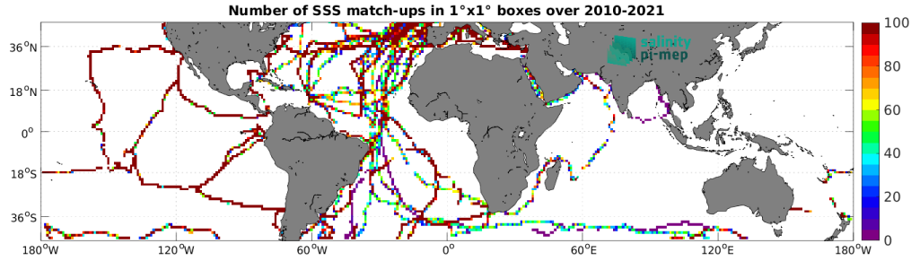
Figure 5: Number of SSS match-ups between TSG (GOSUD-Sailing-ship) SSS and the SMOS SSS L4 v1 - Monthly (CMEMS-CNR) SSS product for the Mid-Low Latitudes 45N-45S Pi-MEP region over 1^{\circ} \times 1^{\circ} boxes and for the full satellite product period.
