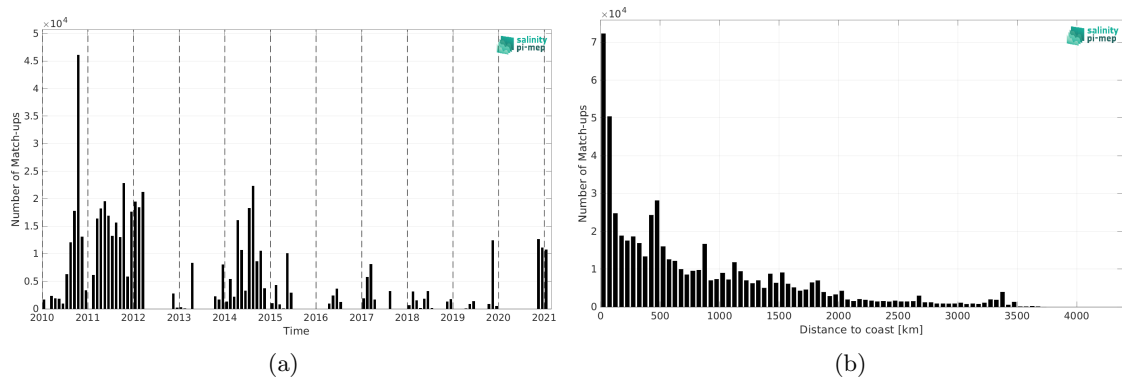
Figure 2: Number of match-ups between TSG (GOSUD-Sailing-ship) and SMOS SSS L4 v1 - Monthly (CMEMS-CNR) SSS as a function of time (a) and as function of the distance to coast (b) over the Mid-Low Latitudes 45N-45S Pi-MEP region and for the full satellite product period.
