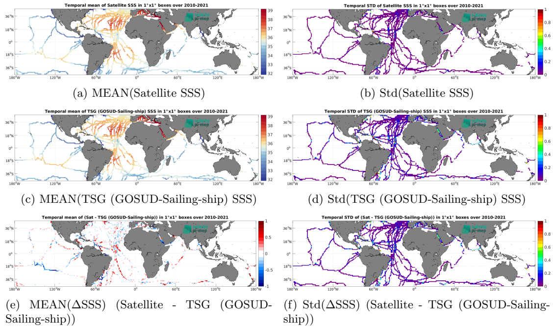
Figure 7: Temporal mean (left) and Std (right) of SSS from SMOS SSS L4 v1 - Monthly (CMEMS-CNR) (top), TSG (GOSUD-Sailing-ship) (middle), and of \Delta SSS (Satellite - TSG (GOSUD-Sailing-ship)). Only match-up pairs are used to generate these maps.
