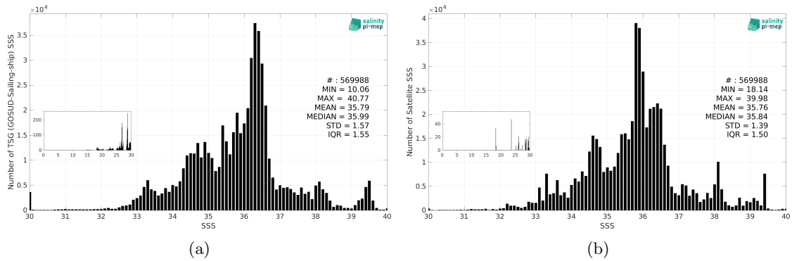
Figure 3: Histograms of SSS from TSG (GOSUD-Sailing-ship) (a) and SMOS SSS L4 v1 - Monthly (CMEMS-CNR) (b) considering all match-up pairs per bins of 0.1 over the Mid-Low Latitudes 45N-45S Pi-MEP region and for the full satellite product period.
