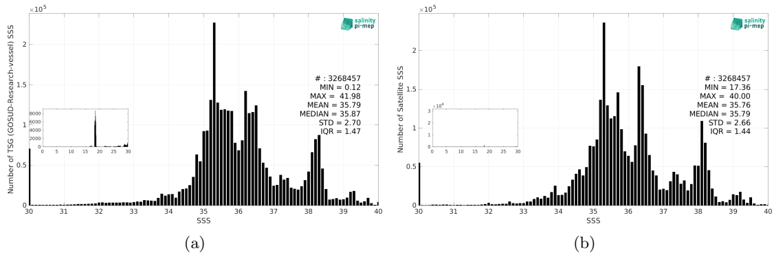
Figure 3: Histograms of SSS from TSG (GOSUD-Research-vessel) (a) and SMOS SSS L4 v1 - Monthly (CMEMS-CNR) (b) considering all match-up pairs per bins of 0.1 over the Mid-Low Latitudes 45N-45S Pi-MEP region and for the full satellite product period.
