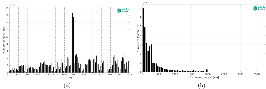
Figure 2: Number of match-ups between TSG (GOSUD-Research-vessel) and SMOS SSS L4 v1 - Monthly (CMEMS-CNR) SSS as a function of time (a) and as function of the distance to coast (b) over the Mid-Low Latitudes 45N-45S Pi-MEP region and for the full satellite product period.
