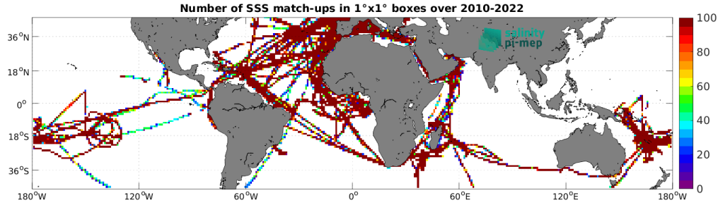
Figure 5: Number of SSS match-ups between TSG (GOSUD-Research-vessel) SSS and the SMOS SSS L4 v1 - Monthly (CMEMS-CNR) SSS product for the Mid-Low Latitudes 45N-45S Pi-MEP region over 1^{\circ} \times 1^{\circ} boxes and for the full satellite product period.
