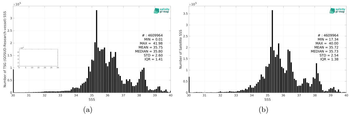
Figure 2: Histograms of SSS from TSG (GOSUD-Research-vessel) (a) and SMOS SSS L4 v1 - Monthly (CMEMS-CNR) (b) considering all match-up pairs per bins of 0.1 over the Mid-Low Latitudes 45N-45S Pi-MEP region and for the full satellite product period.
