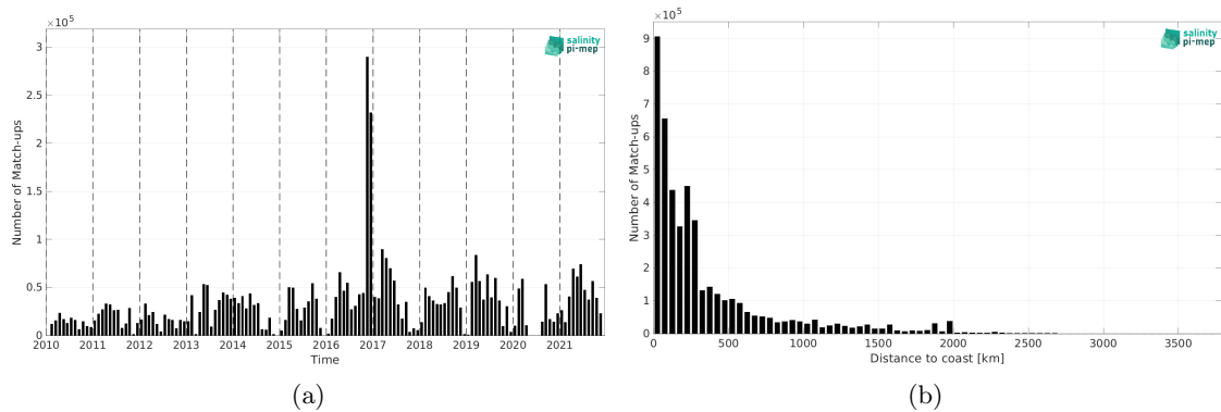
Figure 1: Number of match-ups between TSG (GOSUD-Research-vessel) and SMOS SSS L4 v1 - Monthly (CMEMS-CNR) SSS as a function of time (a) and as function of the distance to coast (b) over the Mid-Low Latitudes 45N-45S Pi-MEP region and for the full satellite product period.
