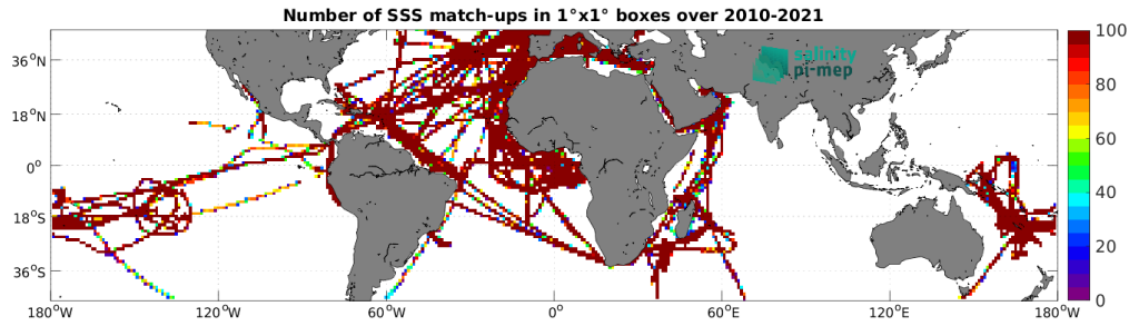
Figure 4: Number of SSS match-ups between TSG (GOSUD-Research-vessel) SSS and the SMOS SSS L4 v1 - Monthly (CMEMS-CNR) SSS product for the Mid-Low Latitudes 45N-45S Pi-MEP region over 1^{\circ} \times 1^{\circ} boxes and for the full satellite product period.
