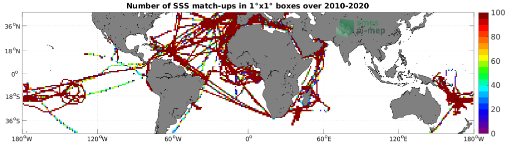
Figure 4: Number of SSS match-ups between TSG (GOSUD-Research-vessel) SSS and the SMOS SSS L4 v1 - Monthly (CMEMS-CNR) SSS product for the Mid-Low Latitudes 45N-45S Pi-MEP region over 1^\circ \times 1^\circ boxes and for the full satellite product period.
