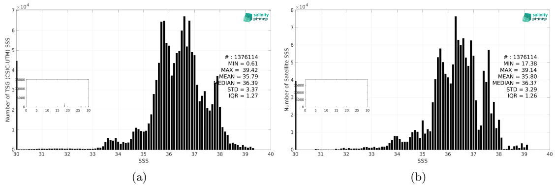
Figure 3: Histograms of SSS from TSG (CSIC-UTM) (a) and SMOS SSS L4 v1 - Monthly (CMEMS-CNR) (b) considering all match-up pairs per bins of 0.1 over the Mid-Low Latitudes 45N-45S Pi-MEP region and for the full satellite product period.
