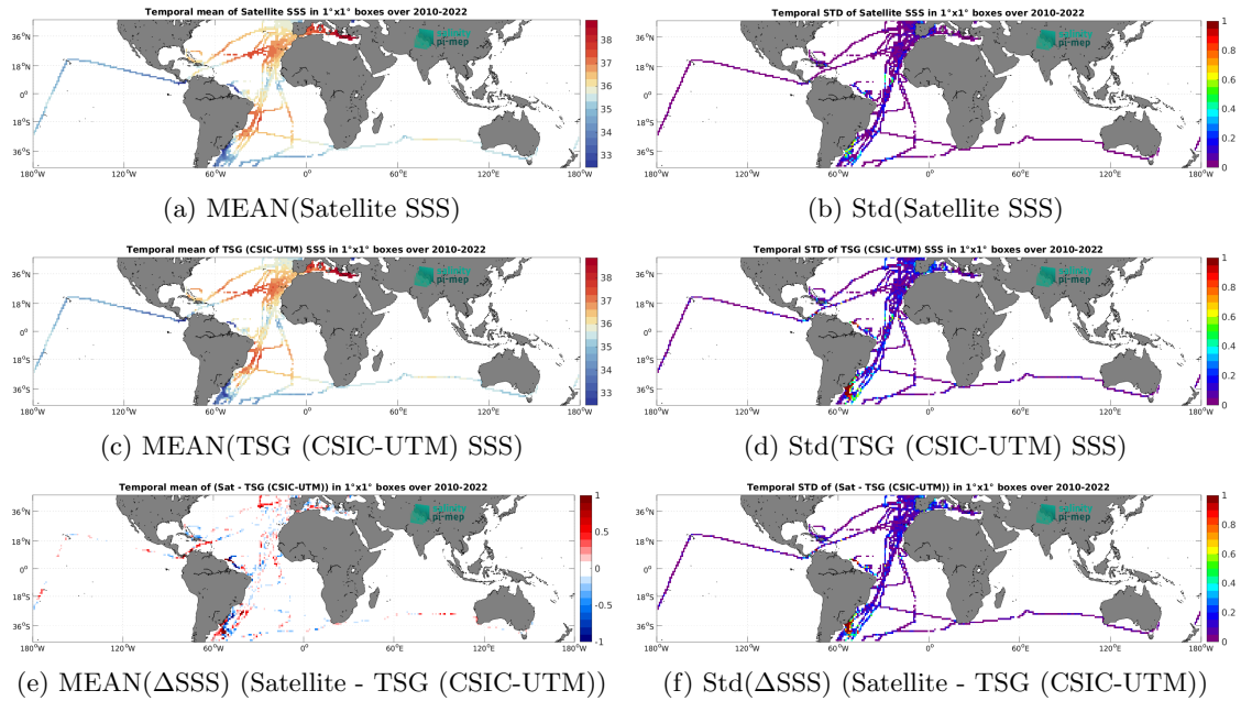
Figure 7: Temporal mean (left) and Std (right) of SSS from SMOS SSS L4 v1 - Monthly (CMEMS-CNR) (top), TSG (CSIC-UTM) (middle), and of \Delta SSS (Satellite - TSG (CSIC-UTM)). Only match-up pairs are used to generate these maps.
