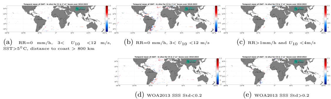
Figure 14: Temporal mean gridded over spatial boxes of size 1^\circ \times 1^\circ of \Delta SSS (SMOS SSS L4 v1 - Monthly (CMEMS-CNR) - TSG (CSIC-UTM)) for 5 different subdatasets corresponding to: RR=0 mm/h, 3 < U_{10} < 12 m/s, SST > 5°C, distance to coast > 800 km (a), RR=0 mm/h, 3 < U_{10} < 12 m/s (b), RR > 1mm/h and U_{10} < 4 m/s (c), WOA2013 SSS Std < 0.2 (d), WOA2013 SSS Std > 0.2 (e).
