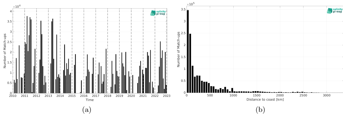
Figure 2: Number of match-ups between TSG (CSIC-UTM) and SMOS SSS L4 v1 - Monthly (CMEMS-CNR) SSS as a function of time (a) and as function of the distance to coast (b) over the Mid-Low Latitudes 45N-45S Pi-MEP region and for the full satellite product period.
