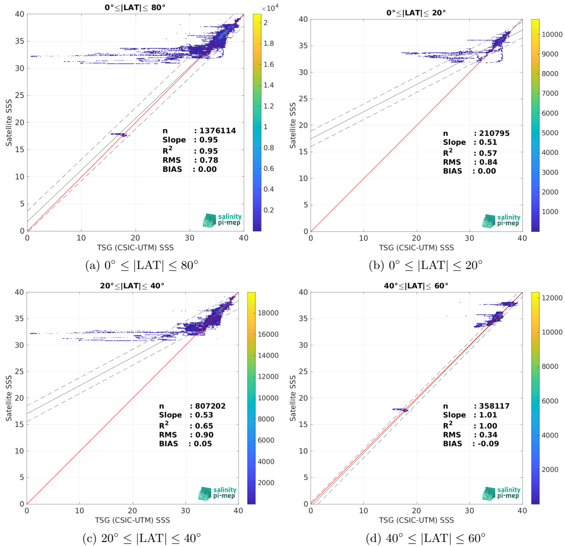
Figure 10: Contour maps of the concentration of SMOS SSS L4 v1 - Monthly (CMEMS-CNR) SSS (y-axis) versus TSG (CSIC-UTM) SSS (x-axis) at match-up pairs for different latitude bands. For each plot, the red line shows x=y . The black thin and dashed lines indicate a linear fit through the data cloud and the \pm 95\% confidence levels, respectively. The number match-up pairs n , the slope and R^2 coefficient of the linear fit, the root mean square (RMS) and the mean bias between satellite and in situ data are indicated for each latitude band in each plots.
