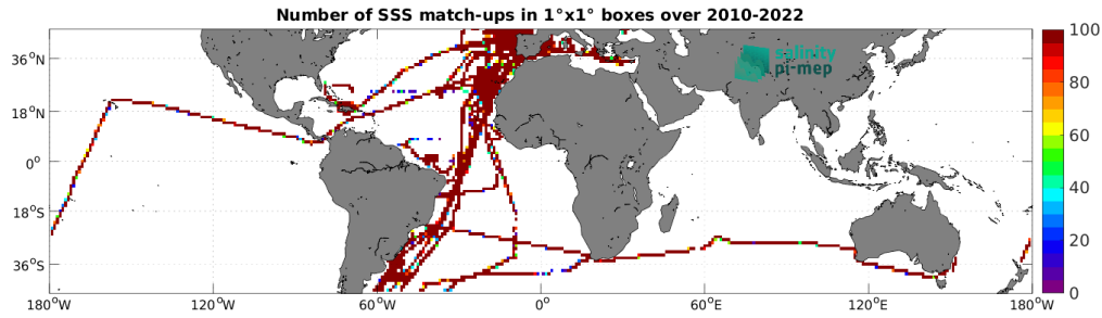
Figure 5: Number of SSS match-ups between TSG (CSIC-UTM) SSS and the SMOS SSS L4 v1 - Monthly (CMEMS-CNR) SSS product for the Mid-Low Latitudes 45N-45S Pi-MEP region over 1^\circ \times 1^\circ boxes and for the full satellite product period.
