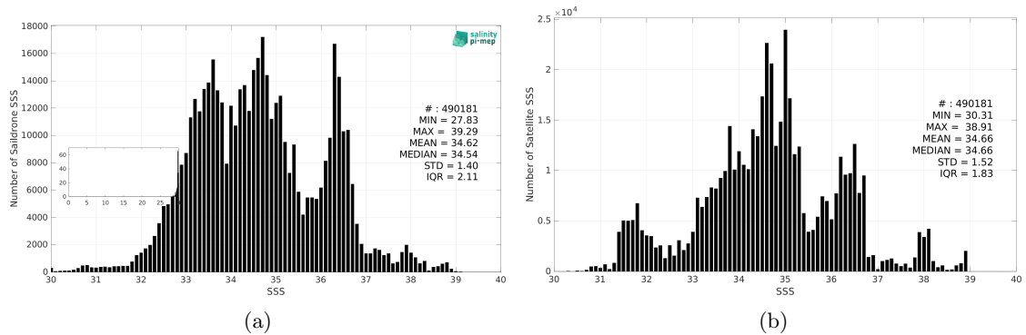
Figure 3: Histograms of SSS from Saildrone (a) and SMOS SSS L4 v1 - Monthly (CMEMS-CNR) (b) considering all match-up pairs per bins of 0.1 over the Mid-Low Latitudes 45N-45S Pi-MEP region and for the full satellite product period.
