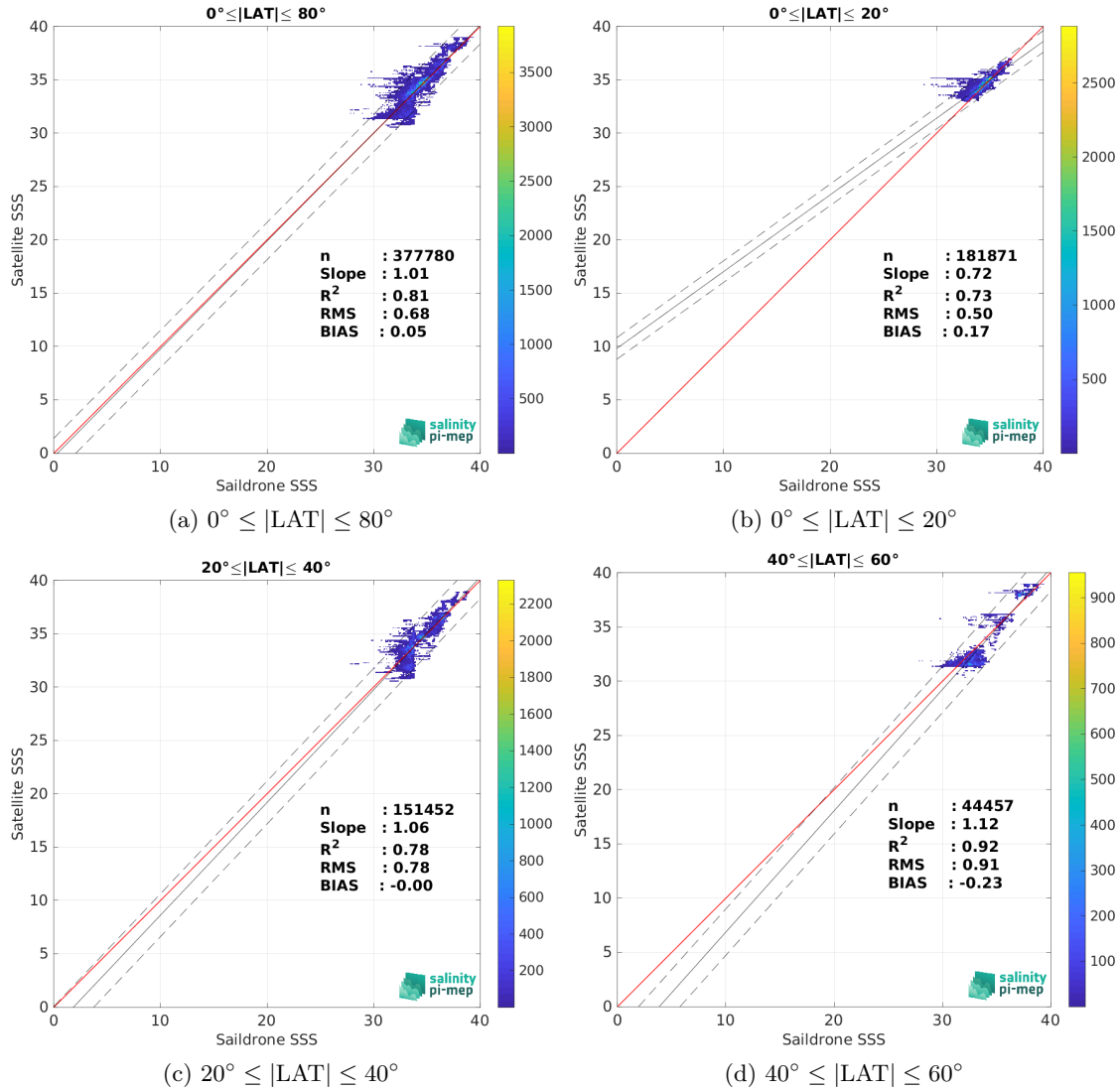
Figure 10: Contour maps of the concentration of SMOS SSS L4 v1 - Monthly (CMEMS-CNR) SSS (y-axis) versus Sairdrone SSS (x-axis) at match-up pairs for different latitude bands. For each plot, the red line shows x=y . The black thin and dashed lines indicate a linear fit through the data cloud and the \pm 95\% confidence levels, respectively. The number match-up pairs n , the slope and R^2 coefficient of the linear fit, the root mean square (RMS) and the mean bias between satellite and in situ data are indicated for each latitude band in each plots.
