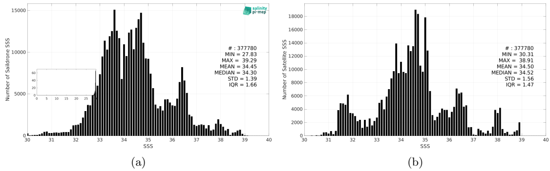
Figure 3: Histograms of SSS from Saildrone (a) and SMOS SSS L4 v1 - Monthly (CMEMS-CNR) (b) considering all match-up pairs per bins of 0.1 over the Mid-Low Latitudes 45N-45S Pi-MEP region and for the full satellite product period.
