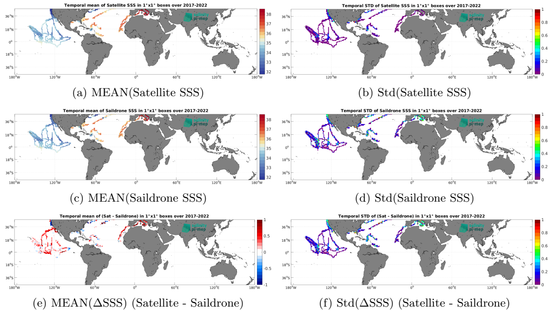
Figure 7: Temporal mean (left) and Std (right) of SSS from SMOS SSS L4 v1 - Monthly (CMEMS-CNR) (top), Saildrone (middle), and of \Delta SSS (Satellite - Saildrone). Only match-up pairs are used to generate these maps.
