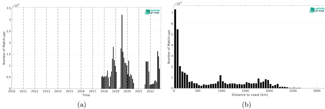
Figure 2: Number of match-ups between Saildrone and SMOS SSS L4 v1 - Monthly (CMEMS-CNR) SSS as a function of time (a) and as function of the distance to coast (b) over the Mid-Low Latitudes 45N-45S Pi-MEP region and for the full satellite product period.
