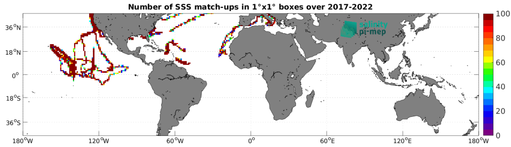
Figure 5: Number of SSS match-ups between Saildrone SSS and the SMOS SSS L4 v1 - Monthly (CMEMS-CNR) SSS product for the Mid-Low Latitudes 45N-45S Pi-MEP region over 1^\circ \times 1^\circ boxes and for the full satellite product period.
