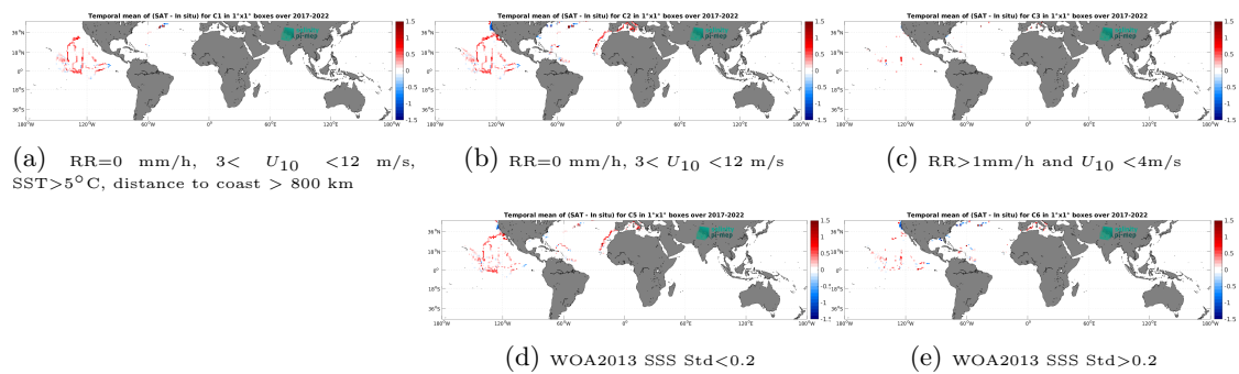
Figure 14: Temporal mean gridded over spatial boxes of size 1^\circ \times 1^\circ of \Delta\text{SSS} (SMOS SSS L4 v1 - Monthly (CMEMS-CNR) - Saldrone) for 5 different subdatasets corresponding to:RR=0 mm/h, 3 < U_{10} < 12 m/s, SST >5^\circ\text{C} , distance to coast > 800 km (a), RR=0 mm/h, 3 < U_{10} < 12 m/s (b), RR >1 mm/h and U_{10} < 4 m/s (c), WOA2013 SSS Std <0.2 (d), WOA2013 SSS Std >0.2 (e).
