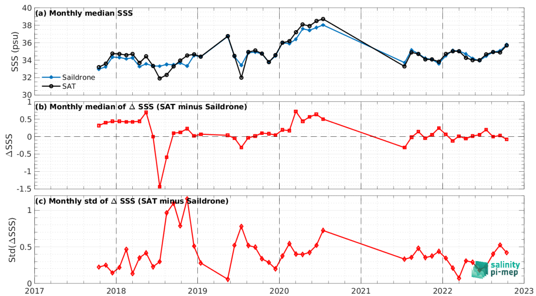
Figure 7: Time series of the monthly median SSS (top), median of \Delta SSS (Satellite - Sairdrone) and Std of \Delta SSS (Satellite - Sairdrone) over the Mid-Low Latitudes 45N-45S Pi-MEP region considering all match-ups collected by the Pi-MEP.
