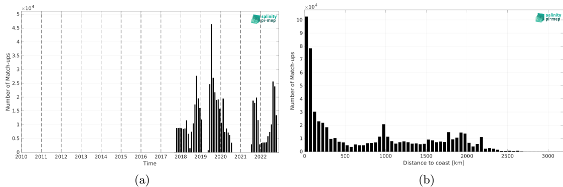
Figure 1: Number of match-ups between Saildrone and SMOS SSS L4 v1 - Monthly (CMEMS-CNR) SSS as a function of time (a) and as function of the distance to coast (b) over the Mid-Low Latitudes 45N-45S Pi-MEP region and for the full satellite product period.
