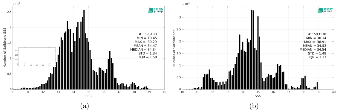
Figure 2: Histograms of SSS from Saildrone (a) and SMOS SSS L4 v1 - Monthly (CMEMS-CNR) (b) considering all match-up pairs per bins of 0.1 over the Mid-Low Latitudes 45N-45S Pi-MEP region and for the full satellite product period.
