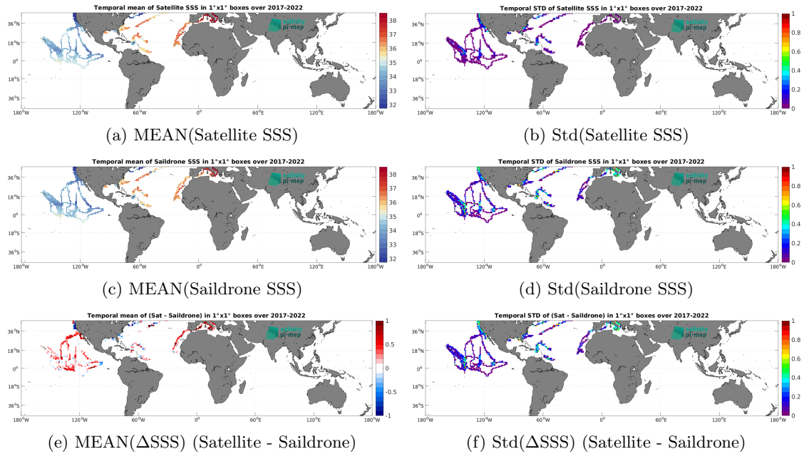
Figure 6: Temporal mean (left) and Std (right) of SSS from SMOS SSS L4 v1 - Monthly (CMEMS-CNR) (top), Saildrone (middle), and of \Delta SSS (Satellite - Saildrone). Only match-up pairs are used to generate these maps.
