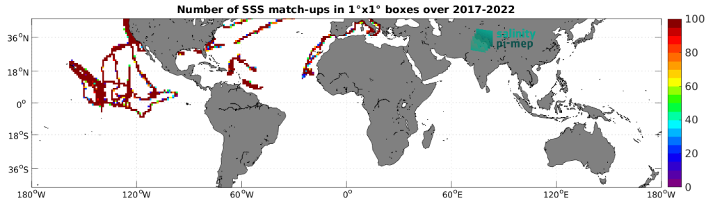
Figure 4: Number of SSS match-ups between Saildrone SSS and the SMOS SSS L4 v1 - Monthly (CMEMS-CNR) SSS product for the Mid-Low Latitudes 45N-45S Pi-MEP region over 1^\circ \times 1^\circ boxes and for the full satellite product period.
