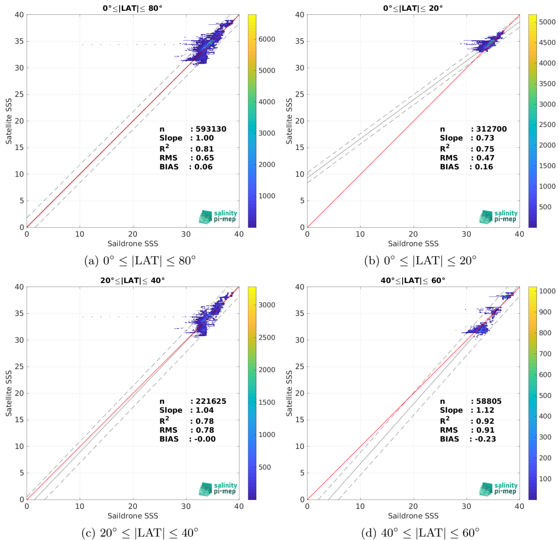
Figure 9: Contour maps of the concentration of SMOS SSS L4 v1 - Monthly (CMEMS-CNR) SSS (y-axis) versus Sairdrone SSS (x-axis) at match-up pairs for different latitude bands. For each plot, the red line shows x=y . The black thin and dashed lines indicate a linear fit through the data cloud and the \pm 95\% confidence levels, respectively. The number match-up pairs n , the slope and R^2 coefficient of the linear fit, the root mean square (RMS) and the mean bias between satellite and in situ data are indicated for each latitude band in each plots.
