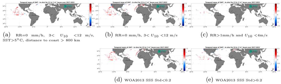
Figure 12: Temporal mean gridded over spatial boxes of size 1^\circ \times 1^\circ of \Delta SSS (SMOS SSS L4 v1 - Monthly (CMEMS-CNR) - Saildrone) for 5 different subdatasets corresponding to: RR=0 mm/h, 3 < U_{10} < 12 m/s, SST >5^\circ\text{C} , distance to coast > 800 km (a), RR=0 mm/h, 3 < U_{10} < 12 m/s (b), RR >1 mm/h and U_{10} < 4 m/s (c), WOA2013 SSS Std <0.2 (d), WOA2013 SSS Std >0.2 (e).
