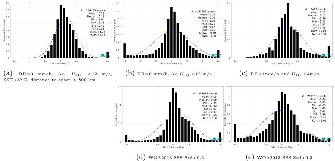
Figure 13: Normalized histogram of \Delta SSS (SMOS SSS L4 v1 - Monthly (CMEMS-CNR) - Saildrone) for 5 different subdatasets corresponding to: RR=0 mm/h, 3 < U_{10} < 12 m/s, SST >5^\circ\text{C} , distance to coast > 800 km (a), RR=0 mm/h, 3 < U_{10} < 12 m/s (b), RR >1 mm/h and U_{10} < 4 m/s (c), WOA2013 SSS Std <0.2 (d), WOA2013 SSS Std >0.2 (e).
