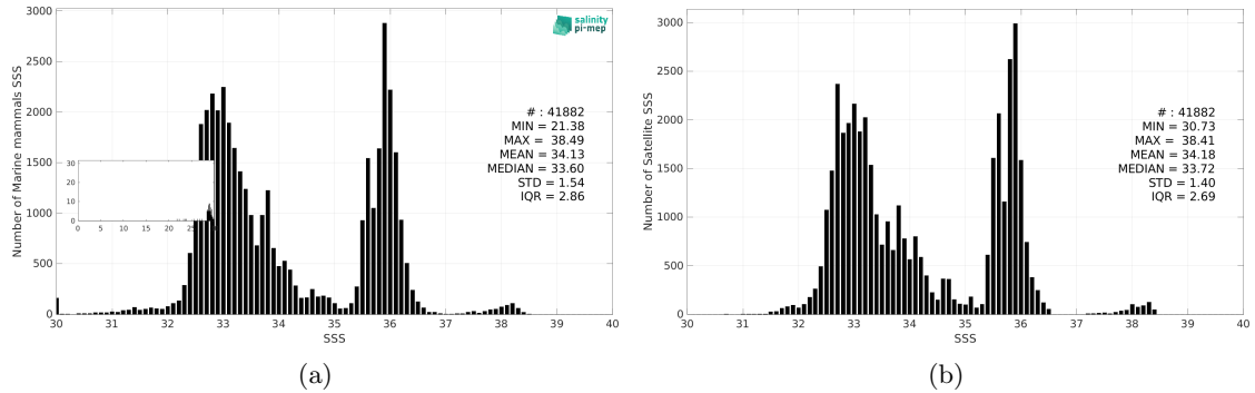
Figure 3: Histograms of SSS from Marine mammals (a) and SMOS SSS L4 v1 - Monthly (CMEMS-CNR) (b) considering all match-up pairs per bins of 0.1 over the Mid-Low Latitudes 45N-45S Pi-MEP region and for the full satellite product period.
