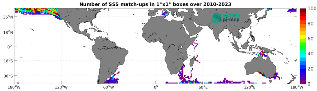
Figure 5: Number of SSS match-ups between Marine mammals SSS and the SMOS SSS L4 v1 - Monthly (CMEMS-CNR) SSS product for the Mid-Low Latitudes 45N-45S Pi-MEP region over 1^\circ \times 1^\circ boxes and for the full satellite product period.
