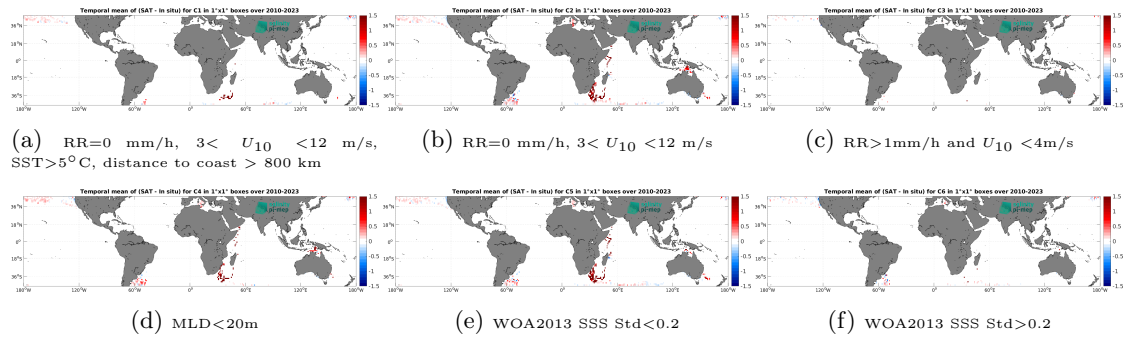
Figure 14: Temporal mean gridded over spatial boxes of size 1^\circ \times 1^\circ of \Delta SSS (SMOS SSS L4 v1 - Monthly (CMEMS-CNR) - Marine mammals) for 6 different subdatasets corresponding to:RR=0 mm/h, 3 < U_{10} < 12 m/s, SST >5^\circ C, distance to coast > 800 km (a), RR=0 mm/h, 3 < U_{10} < 12 m/s (b), RR >1 mm/h and U_{10} < 4 m/s (c),MLD <20 m (d),WOA2013 SSS Std <0.2 (e),WOA2013 SSS Std >0.2 (f).
