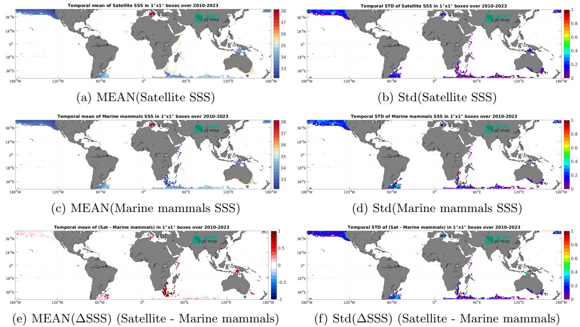
Figure 7: Temporal mean (left) and Std (right) of SSS from SMOS SSS L4 v1 - Monthly (CMEMS-CNR) (top), Marine mammals (middle), and of \Delta SSS (Satellite - Marine mammals). Only match-up pairs are used to generate these maps.
