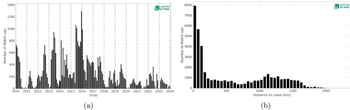
Figure 2: Number of match-ups between Marine mammals and SMOS SSS L4 v1 - Monthly (CMEMS-CNR) SSS as a function of time (a) and as function of the distance to coast (b) over the Mid-Low Latitudes 45N-45S Pi-MEP region and for the full satellite product period.
