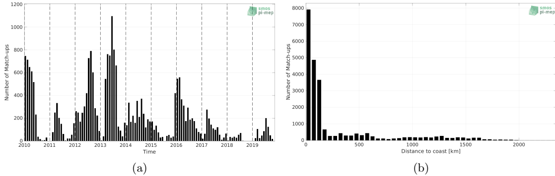
Figure 1: Number of match-ups between Marine mammals and SMOS SSS L4 v1 - Monthly (CMEMS-CNR) SSS as a function of time (a) and as function of the distance to coast (b) over the Mid-Low Latitudes 45N-45S Pi-MEP region and for the full satellite product period.
