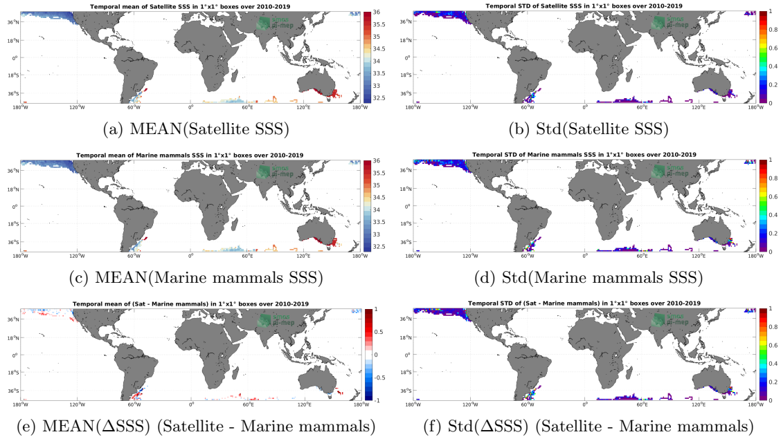
Figure 6: Temporal mean (left) and Std (right) of SSS from SMOS SSS L4 v1 - Monthly (CMEMS-CNR) (top), Marine mammals (middle), and of \Delta SSS (Satellite - Marine mammals). Only match-up pairs are used to generate these maps.
