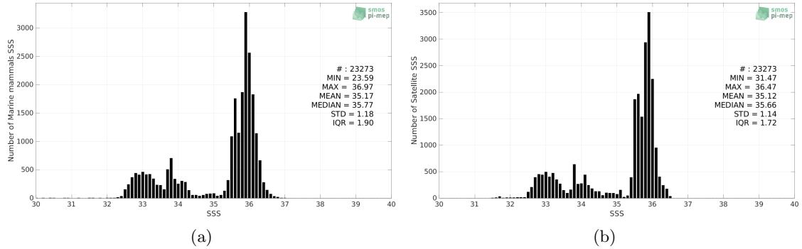
Figure 2: Histograms of SSS from Marine mammals (a) and SMOS SSS L4 v1 - Monthly (CMEMS-CNR) (b) considering all match-up pairs per bins of 0.1 over the Mid-Low Latitudes 45N-45S Pi-MEP region and for the full satellite product period.
