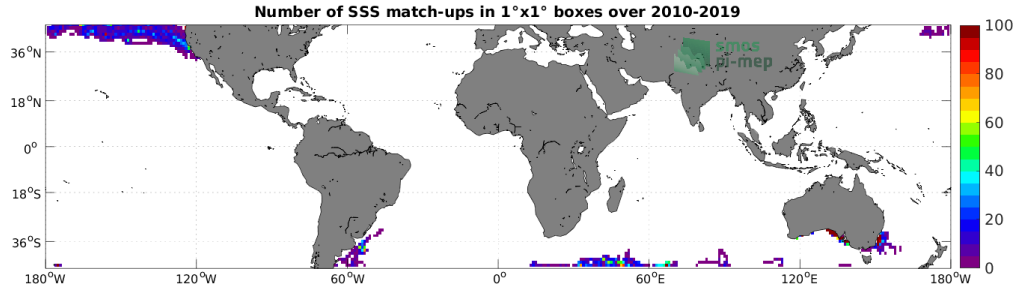
Figure 4: Number of SSS match-ups between Marine mammals SSS and the SMOS SSS L4 v1 - Monthly (CMEMS-CNR) SSS product for the Mid-Low Latitudes 45N-45S Pi-MEP region over 1^\circ \times 1^\circ boxes and for the full satellite product period.
