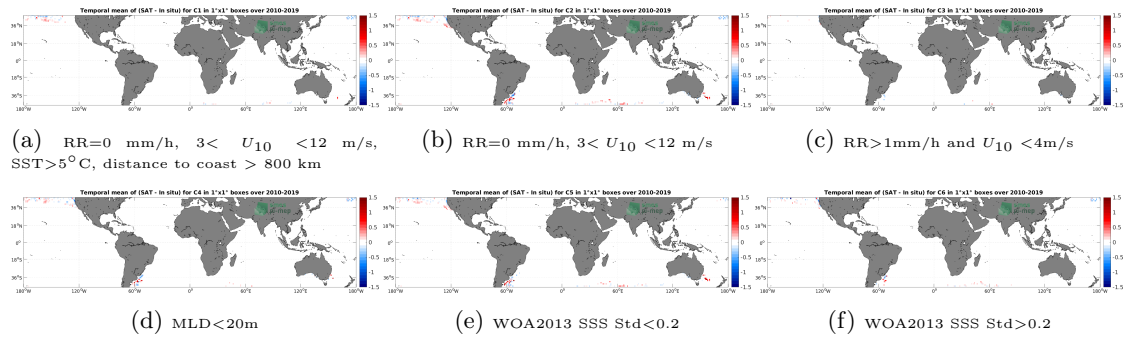
Figure 12: Temporal mean gridded over spatial boxes of size 1^\circ \times 1^\circ of \Delta SSS (SMOS SSS L4 v1 - Monthly (CMEMS-CNR) - Marine mammals) for 6 different subdatasets corresponding to:RR=0 mm/h, 3 < U_{10} < 12 m/s, SST >5^\circ C, distance to coast > 800 km (a), RR=0 mm/h, 3 < U_{10} < 12 m/s (b), RR >1 mm/h and U_{10} < 4 m/s (c),MLD <20 m (d),WOA2013 SSS Std <0.2 (e),WOA2013 SSS Std >0.2 (f).
