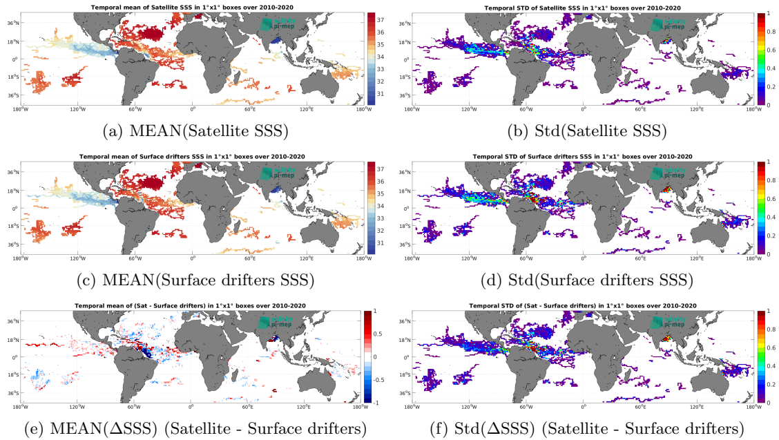
Figure 6: Temporal mean (left) and Std (right) of SSS from SMOS SSS L4 v1 - Monthly (CMEMS-CNR) (top), Surface drifters (middle), and of \Delta SSS (Satellite - Surface drifters). Only match-up pairs are used to generate these maps.
