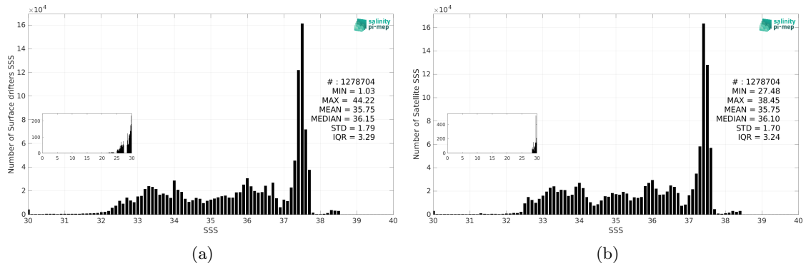
Figure 3: Histograms of SSS from Surface drifters (a) and SMOS SSS L4 v1 - Monthly (CMEMS-CNR) (b) considering all match-up pairs per bins of 0.1 over the Mid-Low Latitudes 45N-45S Pi-MEP region and for the full satellite product period.
