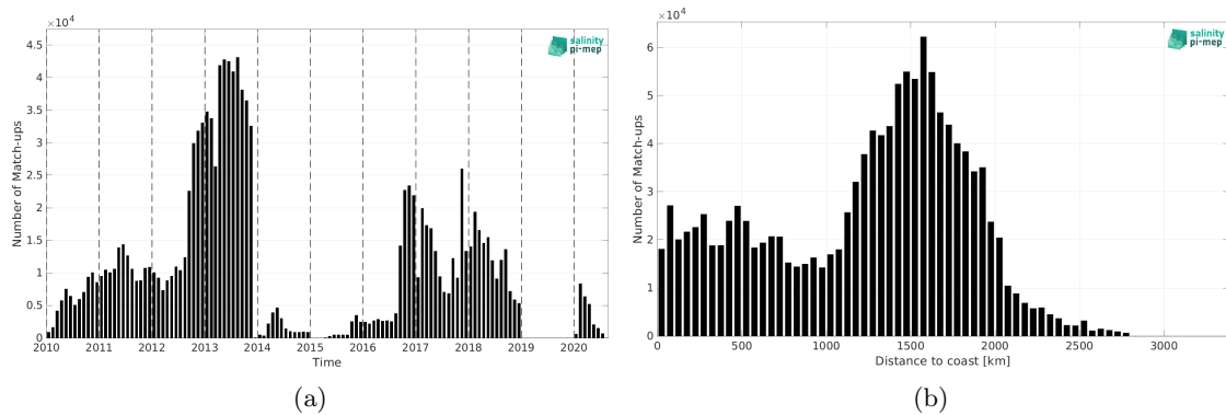
Figure 2: Number of match-ups between Surface drifters and SMOS SSS L4 v1 - Monthly (CMEMS-CNR) SSS as a function of time (a) and as function of the distance to coast (b) over the Mid-Low Latitudes 45N-45S Pi-MEP region and for the full satellite product period.
