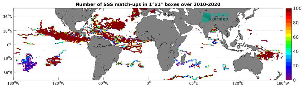
Figure 4: Number of SSS match-ups between Surface drifters SSS and the SMOS SSS L4 v1 - Monthly (CMEMS-CNR) SSS product for the Mid-Low Latitudes 45N-45S Pi-MEP region over 1^\circ \times 1^\circ boxes and for the full satellite product period.
