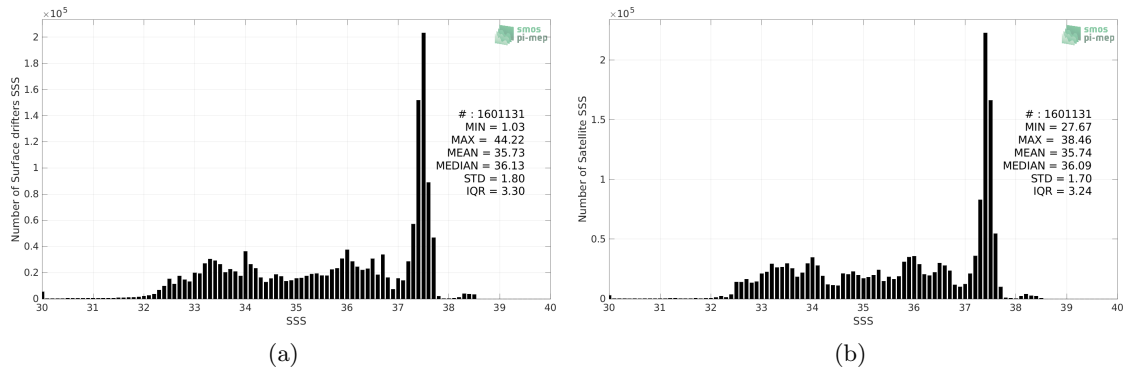
Figure 2: Histograms of SSS from Surface drifters (a) and SMOS SSS L4 v1 - Monthly (CMEMS-CNR) (b) considering all match-up pairs per bins of 0.1 over the Mid-Low Latitudes 45N-45S Pi-MEP region and for the full satellite product period.
