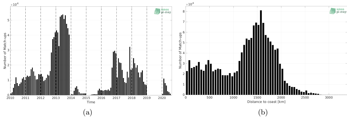
Figure 1: Number of match-ups between Surface drifters and SMOS SSS L4 v1 - Monthly (CMEMS-CNR) SSS as a function of time (a) and as function of the distance to coast (b) over the Mid-Low Latitudes 45N-45S Pi-MEP region and for the full satellite product period.
