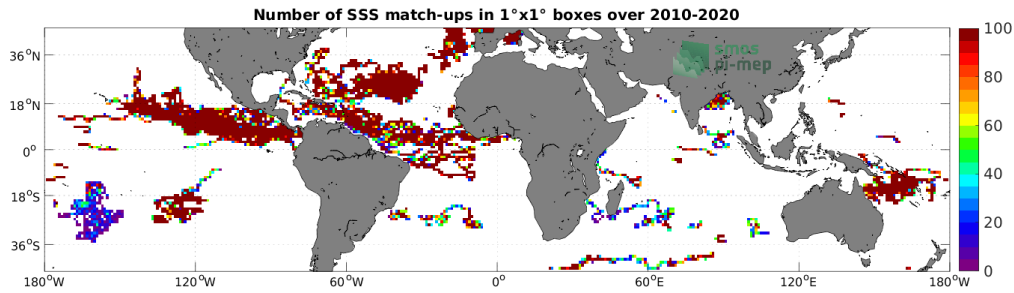
Figure 3: Number of SSS match-ups between Surface drifters SSS and the SMOS SSS L4 v1 - Monthly (CMEMS-CNR) SSS product for the Mid-Low Latitudes 45N-45S Pi-MEP region over 1^\circ \times 1^\circ boxes and for the full satellite product period.
