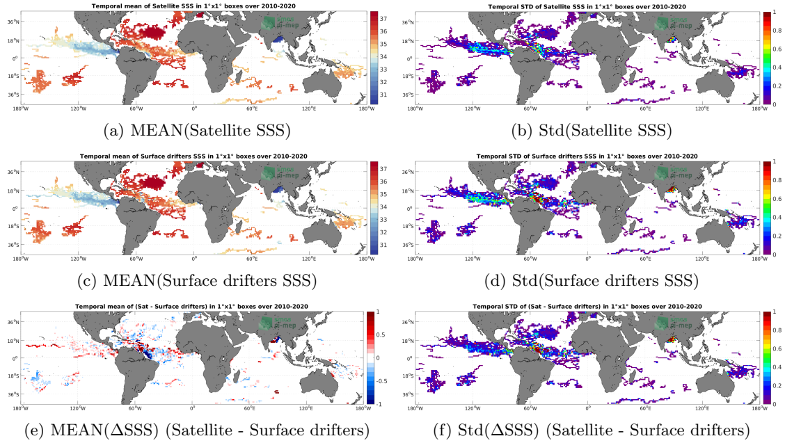
Figure 5: Temporal mean (left) and Std (right) of SSS from SMOS SSS L4 v1 - Monthly (CMEMS-CNR) (top), Surface drifters (middle), and of \Delta SSS (Satellite - Surface drifters). Only match-up pairs are used to generate these maps.
