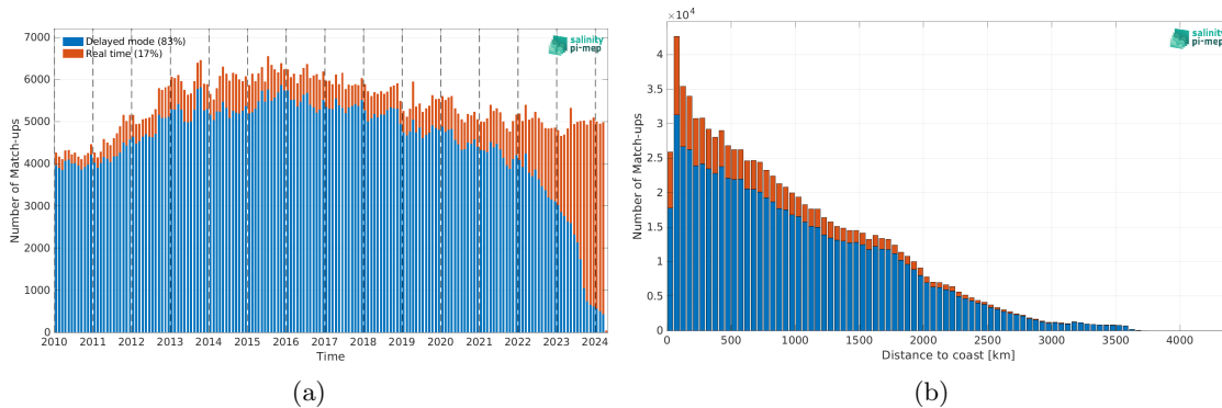
Figure 2: Number of match-ups between Argo and SMOS SSS L4 v1 - Monthly (CMEMS-CNR) SSS as a function of time (a) and as function of the distance to coast (b) over the Mid-Low Latitudes 45N-45S Pi-MEP region and for the full satellite product period.
