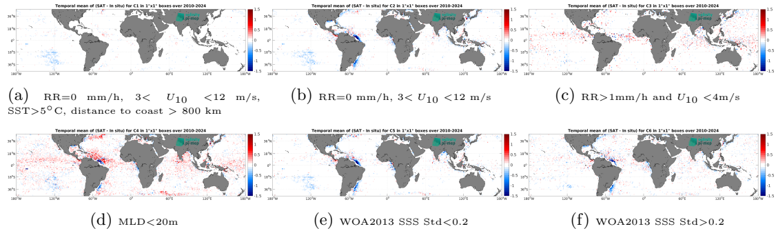
Figure 14: Temporal mean gridded over spatial boxes of size 1^\circ \times 1^\circ of \Delta SSS (SMOS SSS L4 v1 - Monthly (CMEMS-CNR) - Argo) for 6 different subdatasets corresponding to:RR=0 mm/h, 3 < U_{10} < 12 m/s, SST>5°C, distance to coast > 800 km (a), RR=0 mm/h, 3 < U_{10} < 12 m/s (b), RR>1mm/h and U_{10} < 4 m/s (c),MLD<20m (d),WOA2013 SSS Std<0.2 (e),WOA2013 SSS Std>0.2 (f).
