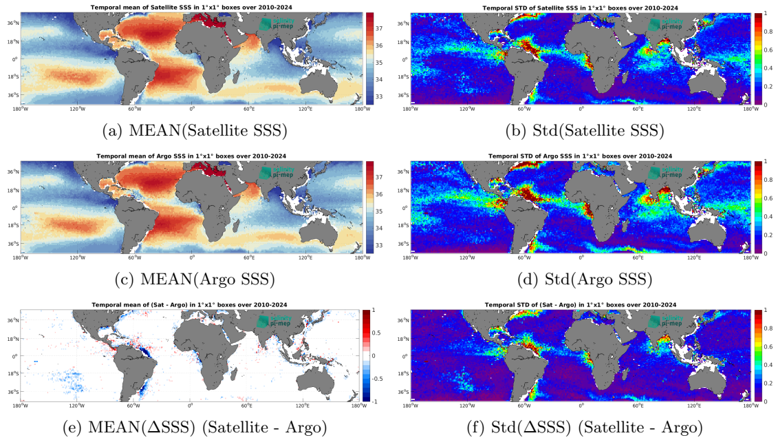
Figure 7: Temporal mean (left) and Std (right) of SSS from SMOS SSS L4 v1 - Monthly (CMEMS-CNR) (top), Argo (middle), and of \Delta SSS (Satellite - Argo). Only match-up pairs are used to generate these maps.
