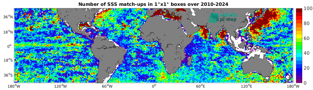
Figure 5: Number of SSS match-ups between Argo SSS and the SMOS SSS L4 v1 - Monthly (CMEMS-CNR) SSS product for the Mid-Low Latitudes 45N-45S Pi-MEP region over 1^\circ \times 1^\circ boxes and for the full satellite product period.
