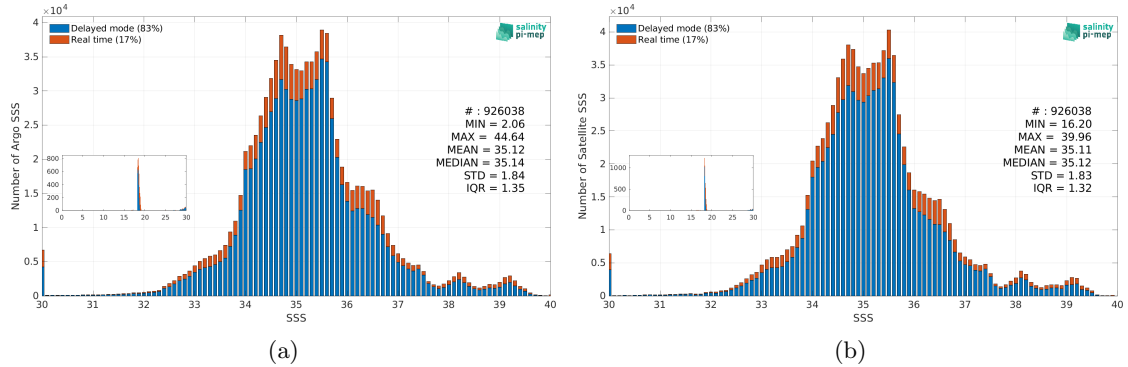
Figure 3: Histograms of SSS from Argo (a) and SMOS SSS L4 v1 - Monthly (CMEMS-CNR) (b) considering all match-up pairs per bins of 0.1 over the Mid-Low Latitudes 45N-45S Pi-MEP region and for the full satellite product period.
