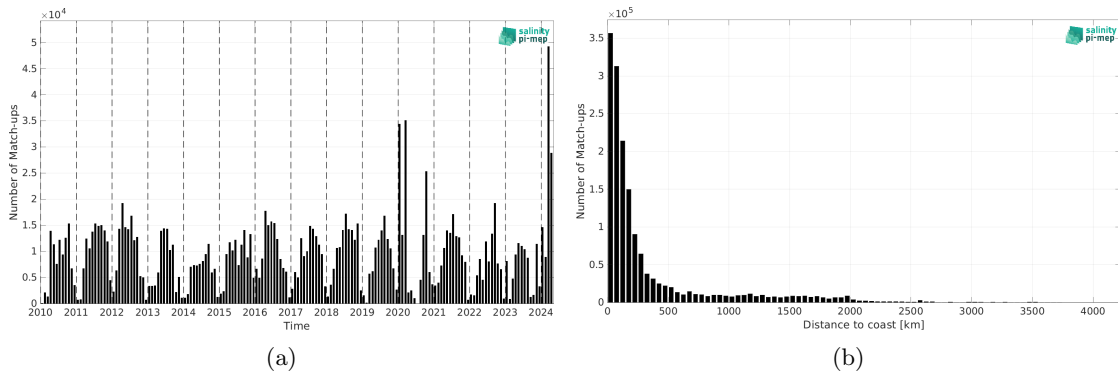
Figure 2: Number of match-ups between TSG (SAMOS) and SMOS SSS L4 v1 - Daily (CMEMS-CNR) SSS as a function of time (a) and as function of the distance to coast (b) over the Mid-Low Latitudes 45N-45S Pi-MEP region and for the full satellite product period.
