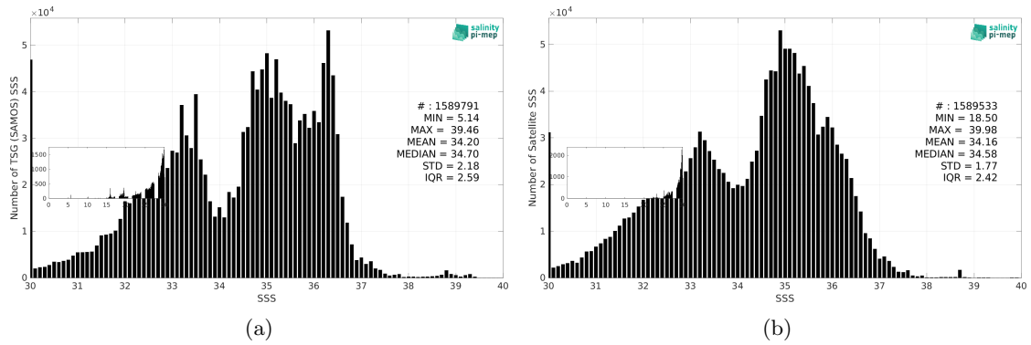
Figure 3: Histograms of SSS from TSG (SAMOS) (a) and SMOS SSS L4 v1 - Daily (CMEMS-CNR) (b) considering all match-up pairs per bins of 0.1 over the Mid-Low Latitudes 45N-45S Pi-MEP region and for the full satellite product period.
