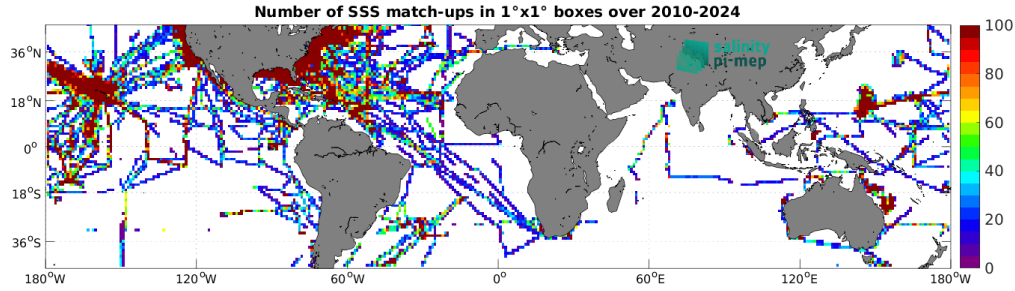
Figure 5: Number of SSS match-ups between TSG (SAMOS) SSS and the SMOS SSS L4 v1 - Daily (CMEMS-CNR) SSS product for the Mid-Low Latitudes 45N-45S Pi-MEP region over 1^\circ \times 1^\circ boxes and for the full satellite product period.
