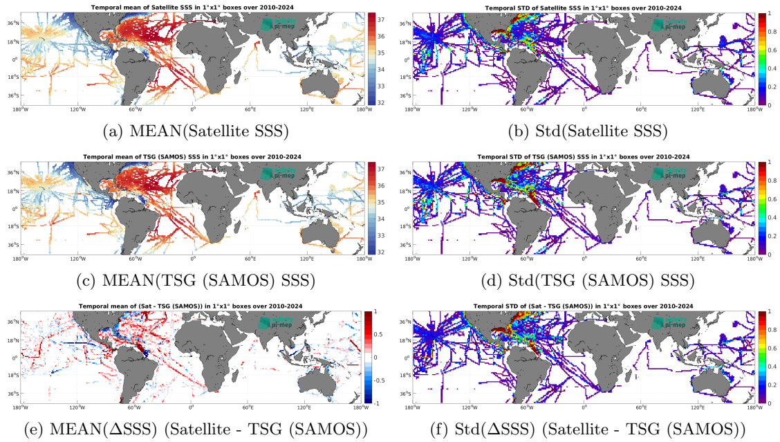
Figure 7: Temporal mean (left) and Std (right) of SSS from SMOS SSS L4 v1 - Daily (CMEMS-CNR) (top), TSG (SAMOS) (middle), and of \Delta SSS (Satellite - TSG (SAMOS)). Only match-up pairs are used to generate these maps.
