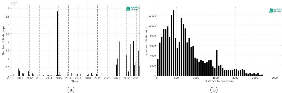
Figure 2: Number of match-ups between TSG (Polarstern) and SMOS SSS L4 v1 - Daily (CMEMS-CNR) SSS as a function of time (a) and as function of the distance to coast (b) over the Mid-Low Latitudes 45N-45S Pi-MEP region and for the full satellite product period.
