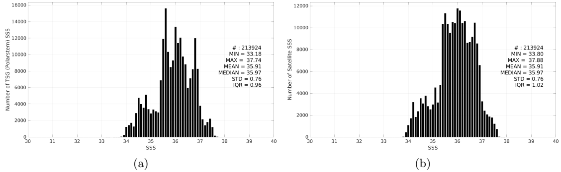
Figure 3: Histograms of SSS from TSG (Polarstern) (a) and SMOS SSS L4 v1 - Daily (CMEMS-CNR) (b) considering all match-up pairs per bins of 0.1 over the Mid-Low Latitudes 45N-45S Pi-MEP region and for the full satellite product period.
