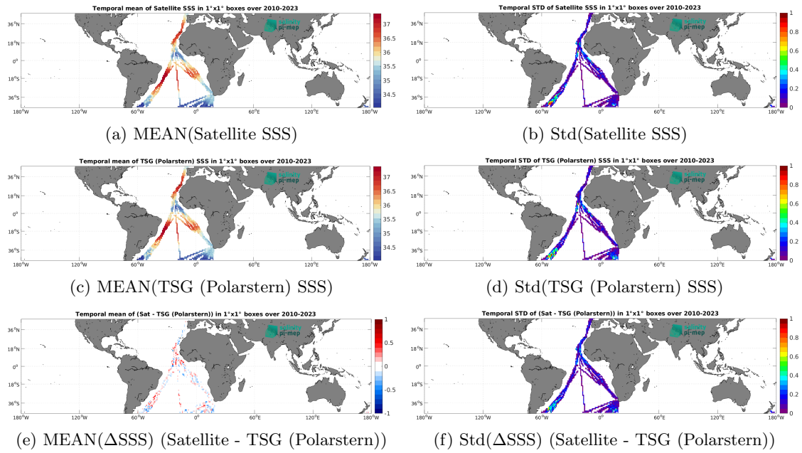
Figure 7: Temporal mean (left) and Std (right) of SSS from SMOS SSS L4 v1 - Daily (CMEMS-CNR) (top), TSG (Polarstern) (middle), and of \Delta SSS (Satellite - TSG (Polarstern)). Only match-up pairs are used to generate these maps.
