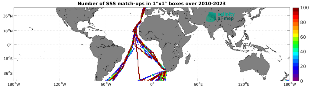
Figure 5: Number of SSS match-ups between TSG (Polarstern) SSS and the SMOS SSS L4 v1 - Daily (CMEMS-CNR) SSS product for the Mid-Low Latitudes 45N-45S Pi-MEP region over 1^\circ \times 1^\circ boxes and for the full satellite product period.
