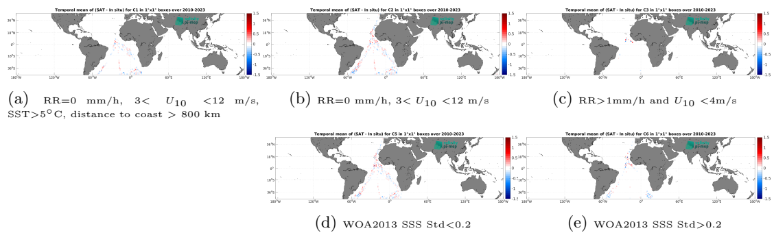
Figure 14: Temporal mean gridded over spatial boxes of size 1^\circ \times 1^\circ of \Delta SSS (SMOS SSS L4 v1 - Daily (CMEMS-CNR) - TSG (Polarstern)) for 5 different subdatasets corresponding to: RR=0 mm/h, 3 < U_{10} < 12 m/s, SST > 5°C, distance to coast > 800 km (a), RR=0 mm/h, 3 < U_{10} < 12 m/s (b), RR > 1mm/h and U_{10} < 4 m/s (c), WOA2013 SSS Std < 0.2 (d), WOA2013 SSS Std > 0.2 (e).
