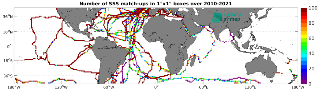
Figure 5: Number of SSS match-ups between TSG (GOSUD-Sailing-ship) SSS and the SMOS SSS L4 v1 - Daily (CMEMS-CNR) SSS product for the Mid-Low Latitudes 45N-45S Pi-MEP region over 1^\circ \times 1^\circ boxes and for the full satellite product period.
