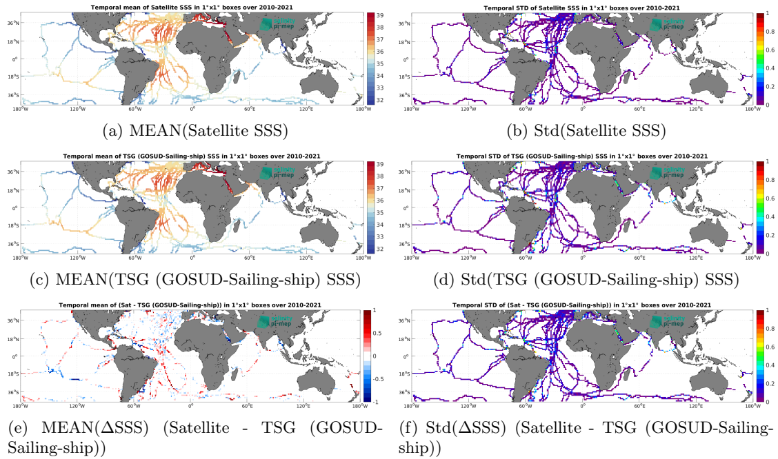
Figure 7: Temporal mean (left) and Std (right) of SSS from SMOS SSS L4 v1 - Daily (CMEMS-CNR) (top), TSG (GOSUD-Sailing-ship) (middle), and of \Delta SSS (Satellite - TSG (GOSUD-Sailing-ship)). Only match-up pairs are used to generate these maps.
