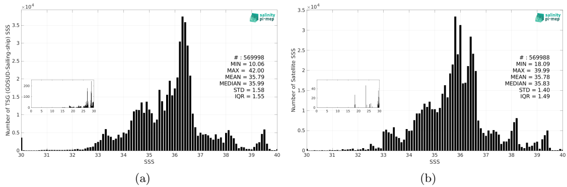
Figure 3: Histograms of SSS from TSG (GOSUD-Sailing-ship) (a) and SMOS SSS L4 v1 - Daily (CMEMS-CNR) (b) considering all match-up pairs per bins of 0.1 over the Mid-Low Latitudes 45N-45S Pi-MEP region and for the full satellite product period.
