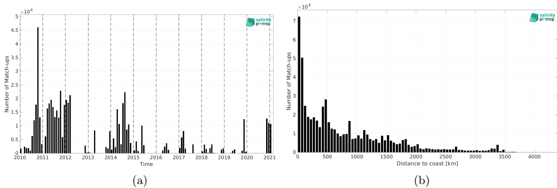
Figure 2: Number of match-ups between TSG (GOSUD-Sailing-ship) and SMOS SSS L4 v1 - Daily (CMEMS-CNR) SSS as a function of time (a) and as function of the distance to coast (b) over the Mid-Low Latitudes 45N-45S Pi-MEP region and for the full satellite product period.
