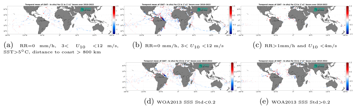
Figure 14: Temporal mean gridded over spatial boxes of size 1^\circ \times 1^\circ of \Delta\text{SSS} (SMOS SSS L4 v1 - Daily (CMEMS-CNR) - TSG (GOSUD-Research-vessel)) for 5 different subdatasets corresponding to:RR=0 mm/h, 3 < U_{10} < 12 m/s, SST>5°C, distance to coast > 800 km (a), RR=0 mm/h, 3 < U_{10} < 12 m/s (b), RR>1mm/h and U_{10} < 4 m/s (c), WOA2013 SSS Std<0.2 (d), WOA2013 SSS Std>0.2 (e).
