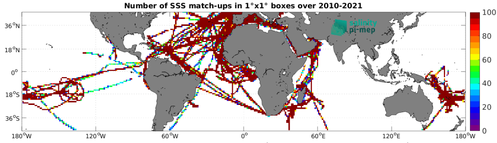
Figure 5: Number of SSS match-ups between TSG (GOSUD-Research-vessel) SSS and the SMOS SSS L4 v1 - Daily (CMEMS-CNR) SSS product for the Mid-Low Latitudes 45N-45S Pi-MEP region over 1^{\circ} \times 1^{\circ} boxes and for the full satellite product period.
