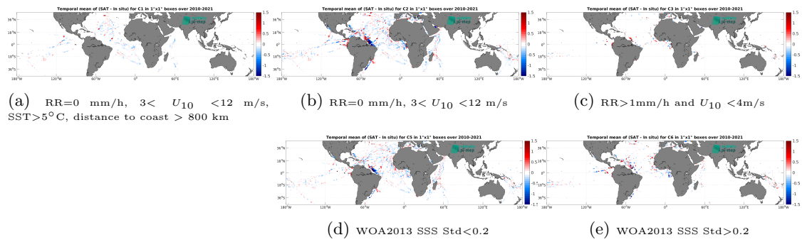
Figure 14: Temporal mean gridded over spatial boxes of size 1^\circ \times 1^\circ of \Delta SSS (SMOS SSS L4 v1 - Daily (CMEMS-CNR) - TSG (GOSUD-Research-vessel)) for 5 different subdatasets corresponding to:RR=0 mm/h, 3 < U_{10} < 12 m/s, SST>5°C, distance to coast > 800 km (a), RR=0 mm/h, 3 < U_{10} < 12 m/s (b), RR>1mm/h and U_{10} < 4 m/s (c), WOA2013 SSS Std<0.2 (d), WOA2013 SSS Std>0.2 (e).
