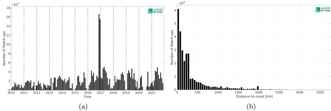
Figure 2: Number of match-ups between TSG (GOSUD-Research-vessel) and SMOS SSS L4 v1 - Daily (CMEMS-CNR) SSS as a function of time (a) and as function of the distance to coast (b) over the Mid-Low Latitudes 45N-45S Pi-MEP region and for the full satellite product period.
