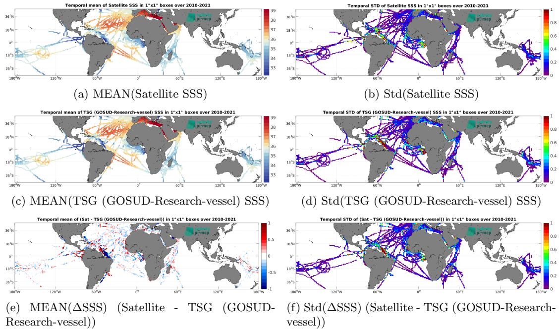
Figure 7: Temporal mean (left) and Std (right) of SSS from SMOS SSS L4 v1 - Daily (CMEMS-CNR) (top), TSG (GOSUD-Research-vessel) (middle), and of \Delta SSS (Satellite - TSG (GOSUD-Research-vessel)). Only match-up pairs are used to generate these maps.
