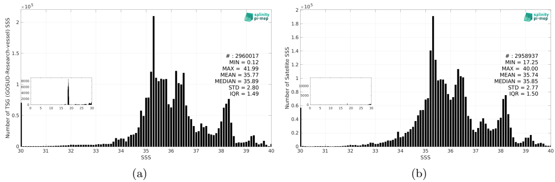
Figure 3: Histograms of SSS from TSG (GOSUD-Research-vessel) (a) and SMOS SSS L4 v1 - Daily (CMEMS-CNR) (b) considering all match-up pairs per bins of 0.1 over the Mid-Low Latitudes 45N-45S Pi-MEP region and for the full satellite product period.
