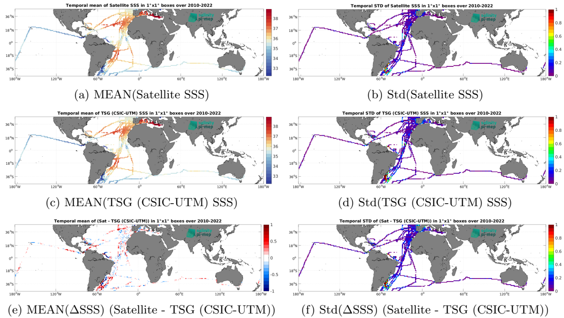
Figure 7: Temporal mean (left) and Std (right) of SSS from SMOS SSS L4 v1 - Daily (CMEMS-CNR) (top), TSG (CSIC-UTM) (middle), and of \Delta SSS (Satellite - TSG (CSIC-UTM)). Only match-up pairs are used to generate these maps.
