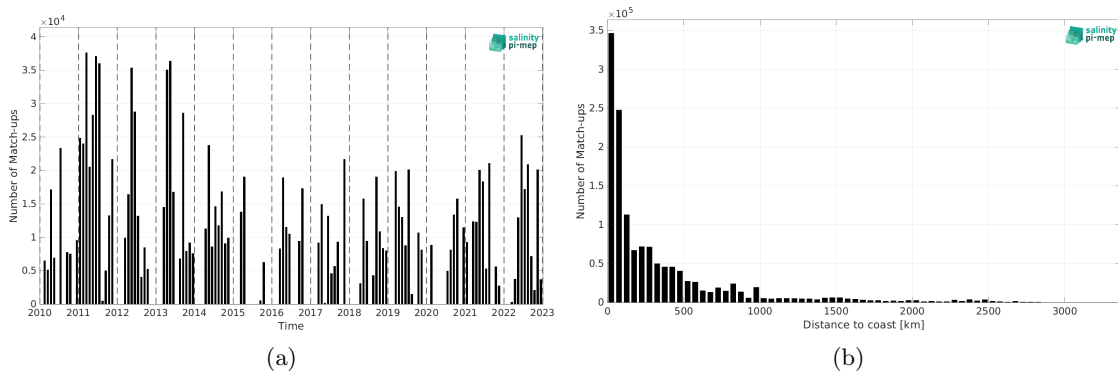
Figure 2: Number of match-ups between TSG (CSIC-UTM) and SMOS SSS L4 v1 - Daily (CMEMS-CNR) SSS as a function of time (a) and as function of the distance to coast (b) over the Mid-Low Latitudes 45N-45S Pi-MEP region and for the full satellite product period.
