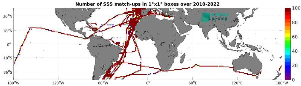
Figure 5: Number of SSS match-ups between TSG (CSIC-UTM) SSS and the SMOS SSS L4 v1 - Daily (CMEMS-CNR) SSS product for the Mid-Low Latitudes 45N-45S Pi-MEP region over 1^\circ \times 1^\circ boxes and for the full satellite product period.
