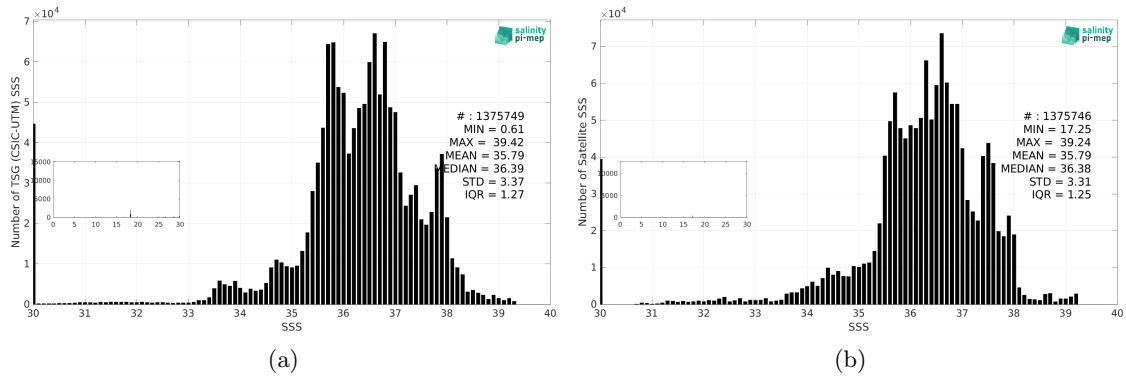
Figure 3: Histograms of SSS from TSG (CSIC-UTM) (a) and SMOS SSS L4 v1 - Daily (CMEMS-CNR) (b) considering all match-up pairs per bins of 0.1 over the Mid-Low Latitudes 45N-45S Pi-MEP region and for the full satellite product period.
