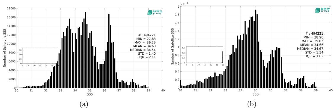
Figure 3: Histograms of SSS from Saildrone (a) and SMOS SSS L4 v1 - Daily (CMEMS-CNR) (b) considering all match-up pairs per bins of 0.1 over the Mid-Low Latitudes 45N-45S Pi-MEP region and for the full satellite product period.
