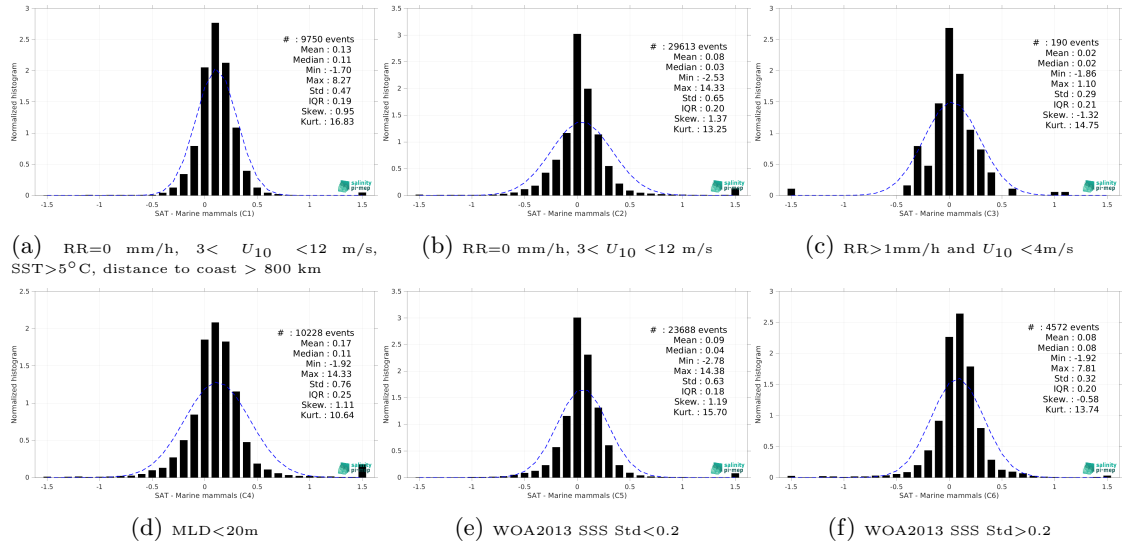
Figure 15: Normalized histogram of \Delta SSS (SMOS SSS L4 v1 - Daily (CMEMS-CNR) - Marine mammals) for 6 different subdatasets corresponding to: RR=0 mm/h, 3 < U_{10} < 12 m/s, SST > 5°C, distance to coast > 800 km (a), RR=0 mm/h, 3 < U_{10} < 12 m/s (b), RR > 1mm/h and U_{10} < 4 m/s (c), MLD < 20m (d), WOA2013 SSS Std < 0.2 (e), WOA2013 SSS Std > 0.2 (f).
