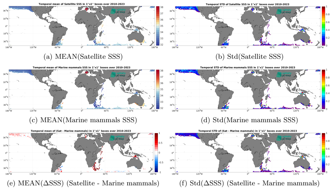
Figure 7: Temporal mean (left) and Std (right) of SSS from SMOS SSS L4 v1 - Daily (CMEMS-CNR) (top), Marine mammals (middle), and of \Delta SSS (Satellite - Marine mammals). Only match-up pairs are used to generate these maps.
