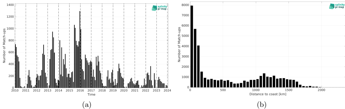
Figure 2: Number of match-ups between Marine mammals and SMOS SSS L4 v1 - Daily (CMEMS-CNR) SSS as a function of time (a) and as function of the distance to coast (b) over the Mid-Low Latitudes 45N-45S Pi-MEP region and for the full satellite product period.
