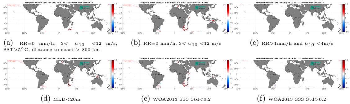
Figure 14: Temporal mean gridded over spatial boxes of size 1^\circ \times 1^\circ of \Delta SSS (SMOS SSS L4 v1 - Daily (CMEMS-CNR) - Marine mammals) for 6 different subdatasets corresponding to:RR=0 mm/h, 3 < U_{10} < 12 m/s, SST > 5°C, distance to coast > 800 km (a), RR=0 mm/h, 3 < U_{10} < 12 m/s (b), RR > 1mm/h and U_{10} < 4 m/s (c),MLD < 20m (d),WOA2013 SSS Std < 0.2 (e),WOA2013 SSS Std > 0.2 (f).
