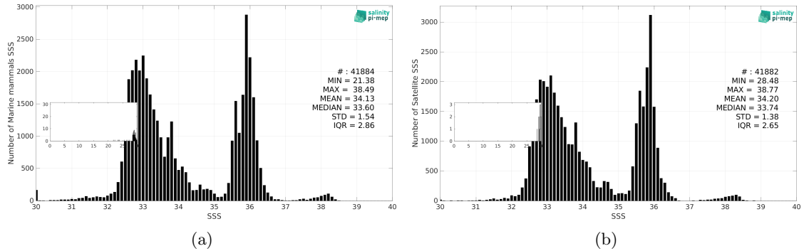
Figure 3: Histograms of SSS from Marine mammals (a) and SMOS SSS L4 v1 - Daily (CMEMS-CNR) (b) considering all match-up pairs per bins of 0.1 over the Mid-Low Latitudes 45N-45S Pi-MEP region and for the full satellite product period.
