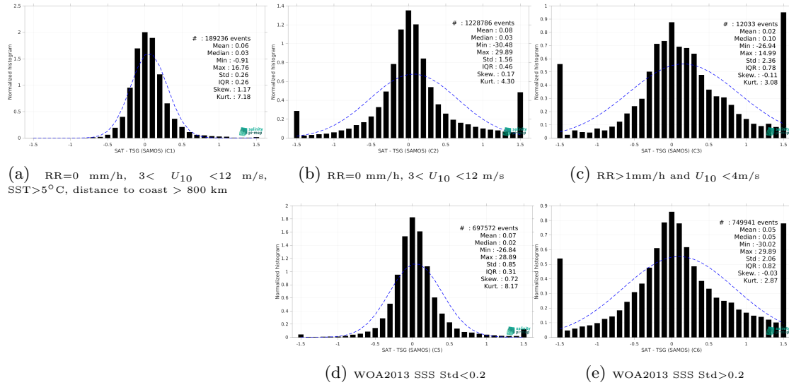
Figure 15: Normalized histogram of \Delta SSS (SMOS SSS L4 OI v346 - Weekly (CMEMS-CATDS-LOPS) - TSG (SAMOS)) for 5 different subdatasets corresponding to: RR=0 mm/h, 3 < U_{10} < 12 m/s, SST > 5°C, distance to coast > 800 km (a), RR=0 mm/h, 3 < U_{10} < 12 m/s (b), RR > 1mm/h and U_{10} < 4 m/s (c), WOA2013 SSS Std < 0.2 (d), WOA2013 SSS Std > 0.2 (e).
