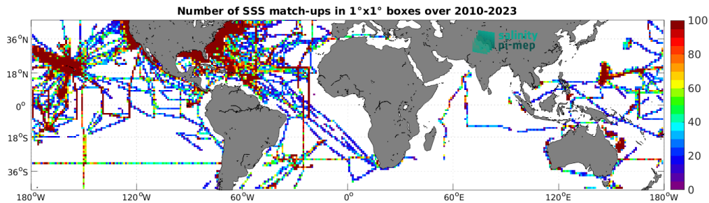
Figure 5: Number of SSS match-ups between TSG (SAMOS) SSS and the SMOS SSS L4 OI v346 - Weekly (CMEMS-CATDS-LOPS) SSS product for the Mid-Low Latitudes 45N-45S Pi-MEP region over 1^\circ \times 1^\circ boxes and for the full satellite product period.
