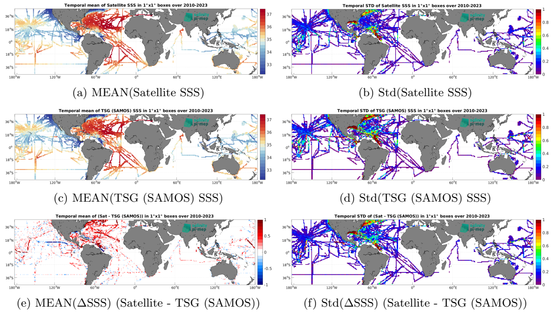
Figure 7: Temporal mean (left) and Std (right) of SSS from SMOS SSS L4 OI v346 - Weekly (CMEMS-CATDS-LOPS) (top), TSG (SAMOS) (middle), and of \Delta SSS (Satellite - TSG (SAMOS)). Only match-up pairs are used to generate these maps.
