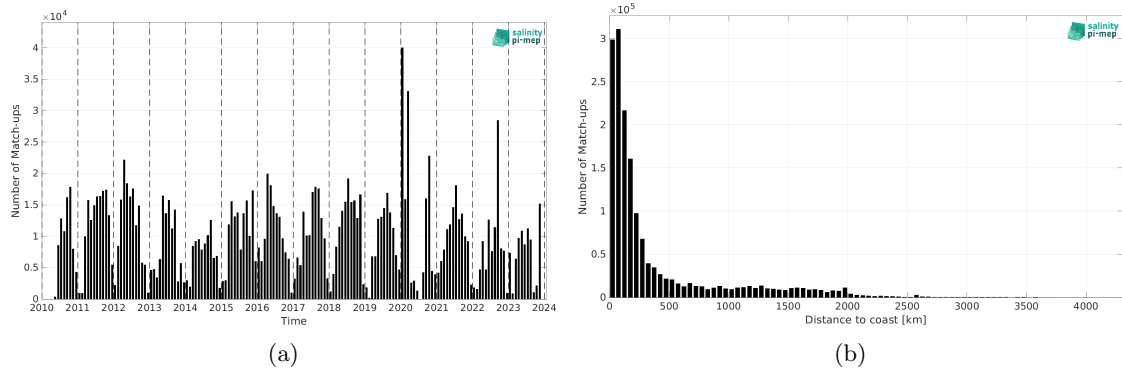
Figure 2: Number of match-ups between TSG (SAMOS) and SMOS SSS L4 OI v346 - Weekly (CMEMS-CATDS-LOPS) SSS as a function of time (a) and as function of the distance to coast (b) over the Mid-Low Latitudes 45N-45S Pi-MEP region and for the full satellite product period.
