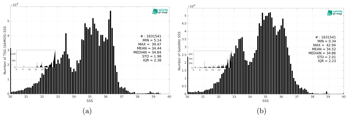
Figure 3: Histograms of SSS from TSG (SAMOS) (a) and SMOS SSS L4 OI v346 - Weekly (CMEMS-CATDS-LOPS) (b) considering all match-up pairs per bins of 0.1 over the Mid-Low Latitudes 45N-45S Pi-MEP region and for the full satellite product period.
