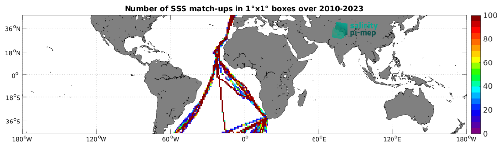
Figure 5: Number of SSS match-ups between TSG (Polarstern) SSS and the SMOS SSS L4 OI v346 - Weekly (CMEMS-CATDS-LOPS) SSS product for the Mid-Low Latitudes 45N-45S Pi-MEP region over 1^\circ \times 1^\circ boxes and for the full satellite product period.
