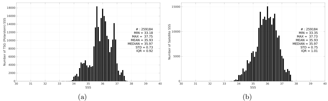
Figure 3: Histograms of SSS from TSG (Polarstern) (a) and SMOS SSS L4 OI v346 - Weekly (CMEMS-CATDS-LOPS) (b) considering all match-up pairs per bins of 0.1 over the Mid-Low Latitudes 45N-45S Pi-MEP region and for the full satellite product period.
