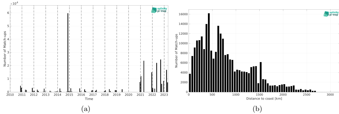
Figure 2: Number of match-ups between TSG (Polarstern) and SMOS SSS L4 OI v346 - Weekly (CMEMS-CATDS-LOPS) SSS as a function of time (a) and as function of the distance to coast (b) over the Mid-Low Latitudes 45N-45S Pi-MEP region and for the full satellite product period.
