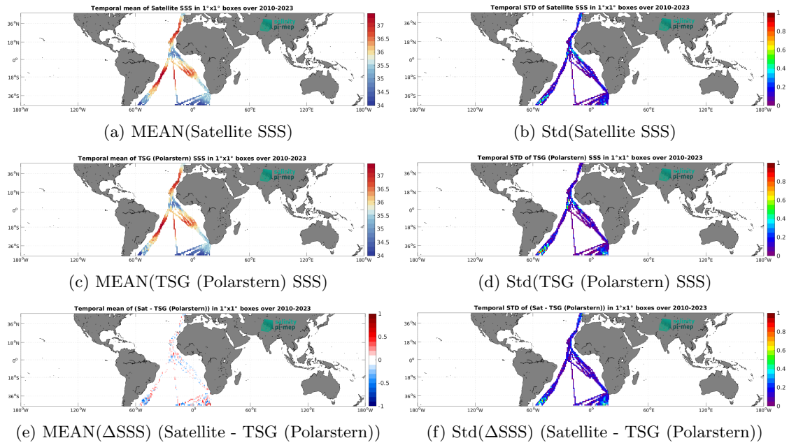
Figure 7: Temporal mean (left) and Std (right) of SSS from SMOS SSS L4 OI v346 - Weekly (CMEMS-CATDS-LOPS) (top), TSG (Polarstern) (middle), and of \Delta SSS (Satellite - TSG (Polarstern)). Only match-up pairs are used to generate these maps.
