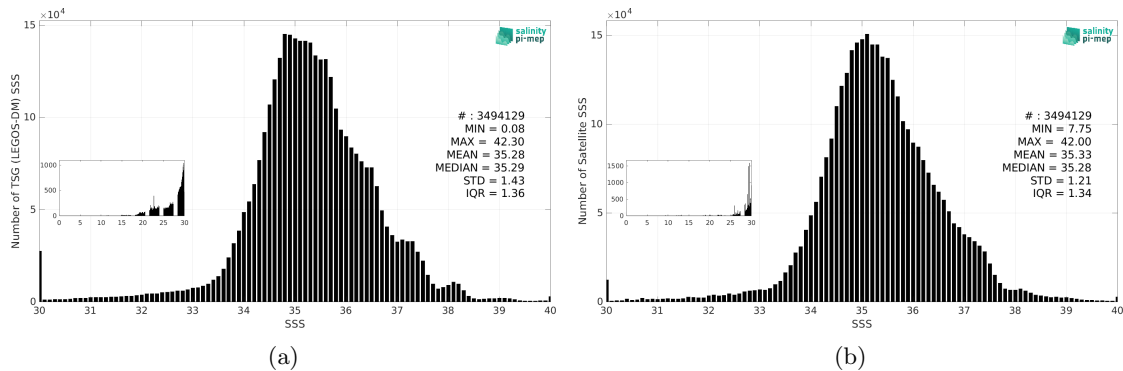
Figure 3: Histograms of SSS from TSG (LEGOS-DM) (a) and SMOS SSS L4 OI v346 - Weekly (CMEMS-CATDS-LOPS) (b) considering all match-up pairs per bins of 0.1 over the Mid-Low Latitudes 45N-45S Pi-MEP region and for the full satellite product period.
