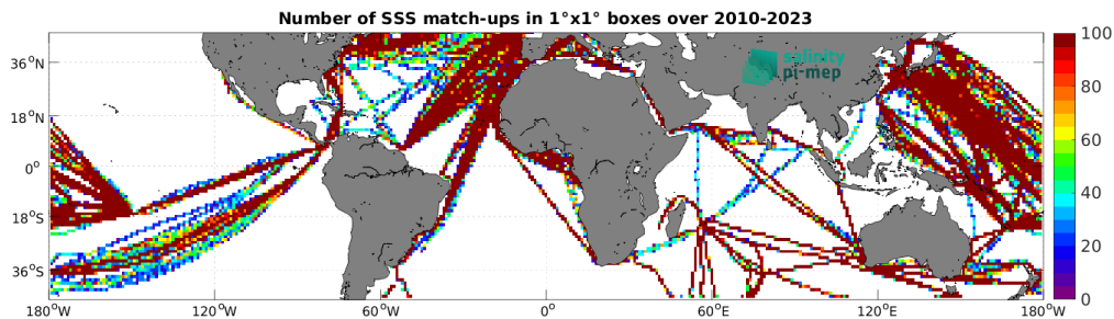
Figure 5: Number of SSS match-ups between TSG (LEGOS-DM) SSS and the SMOS SSS L4 OI v346 - Weekly (CMEMS-CATDS-LOPS) SSS product for the Mid-Low Latitudes 45N-45S Pi-MEP region over 1^\circ \times 1^\circ boxes and for the full satellite product period.
