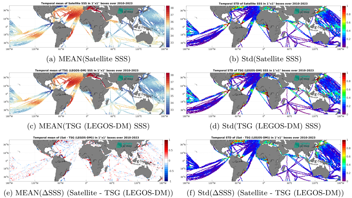
Figure 7: Temporal mean (left) and Std (right) of SSS from SMOS SSS L4 OI v346 - Weekly (CMEMS-CATDS-LOPS) (top), TSG (LEGOS-DM) (middle), and of \Delta SSS (Satellite - TSG (LEGOS-DM)). Only match-up pairs are used to generate these maps.
