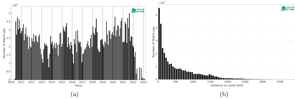
Figure 2: Number of match-ups between TSG (LEGOS-DM) and SMOS SSS L4 OI v346 - Weekly (CMEMS-CATDS-LOPS) SSS as a function of time (a) and as function of the distance to coast (b) over the Mid-Low Latitudes 45N-45S Pi-MEP region and for the full satellite product period.
