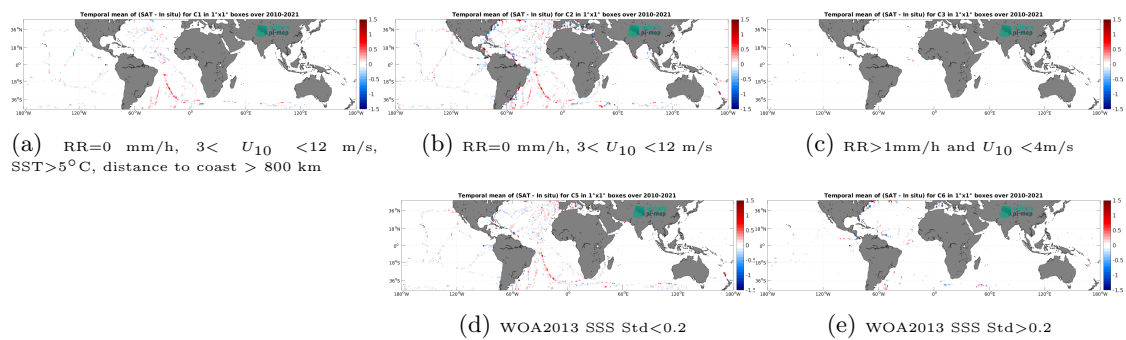
Figure 14: Temporal mean gridded over spatial boxes of size 1^\circ \times 1^\circ of \Delta SSS (SMOS SSS L4 OI v346 - Weekly (CMEMS-CATDS-LOPS) - TSG (GOSUD-Sailing-ship)) for 5 different sub-datasets corresponding to:RR=0 mm/h, 3 < U_{10} < 12 m/s, SST >5^\circ\text{C} , distance to coast > 800 km (a), RR=0 mm/h, 3 < U_{10} < 12 m/s (b), RR >1 mm/h and U_{10} < 4 m/s (c), WOA2013 SSS Std <0.2 (d), WOA2013 SSS Std >0.2 (e).
