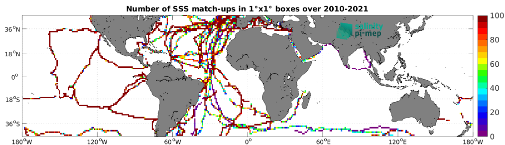
Figure 5: Number of SSS match-ups between TSG (GOSUD-Sailing-ship) SSS and the SMOS SSS L4 OI v346 - Weekly (CMEMS-CATDS-LOPS) SSS product for the Mid-Low Latitudes 45N-45S Pi-MEP region over 1^\circ \times 1^\circ boxes and for the full satellite product period.
