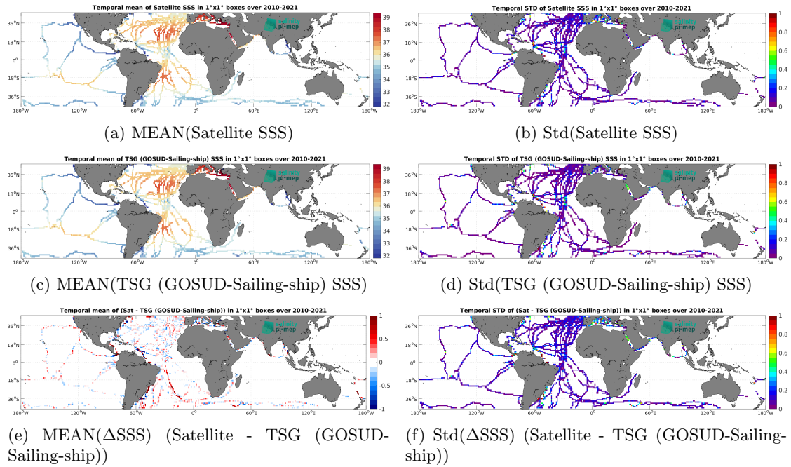
Figure 7: Temporal mean (left) and Std (right) of SSS from SMOS SSS L4 OI v346 - Weekly (CMEMS-CATDS-LOPS) (top), TSG (GOSUD-Sailing-ship) (middle), and of \Delta SSS (Satellite - TSG (GOSUD-Sailing-ship)). Only match-up pairs are used to generate these maps.
