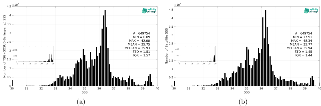
Figure 3: Histograms of SSS from TSG (GOSUD-Sailing-ship) (a) and SMOS SSS L4 OI v346 - Weekly (CMEMS-CATDS-LOPS) (b) considering all match-up pairs per bins of 0.1 over the Mid-Low Latitudes 45N-45S Pi-MEP region and for the full satellite product period.
