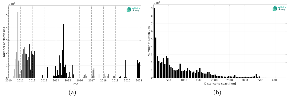
Figure 2: Number of match-ups between TSG (GOSUD-Sailing-ship) and SMOS SSS L4 OI v346 - Weekly (CMEMS-CATDS-LOPS) SSS as a function of time (a) and as function of the distance to coast (b) over the Mid-Low Latitudes 45N-45S Pi-MEP region and for the full satellite product period.
