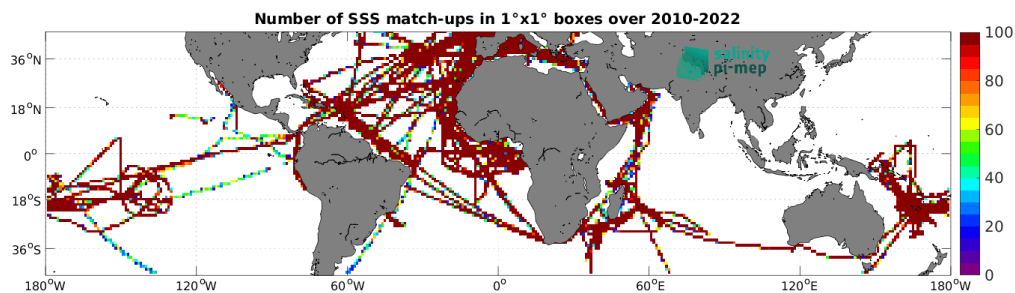
Figure 5: Number of SSS match-ups between TSG (GOSUD-Research-vessel) SSS and the SMOS SSS L4 OI v346 - Weekly (CMEMS-CATDS-LOPS) SSS product for the Mid-Low Latitudes 45N-45S Pi-MEP region over 1^\circ \times 1^\circ boxes and for the full satellite product period.
