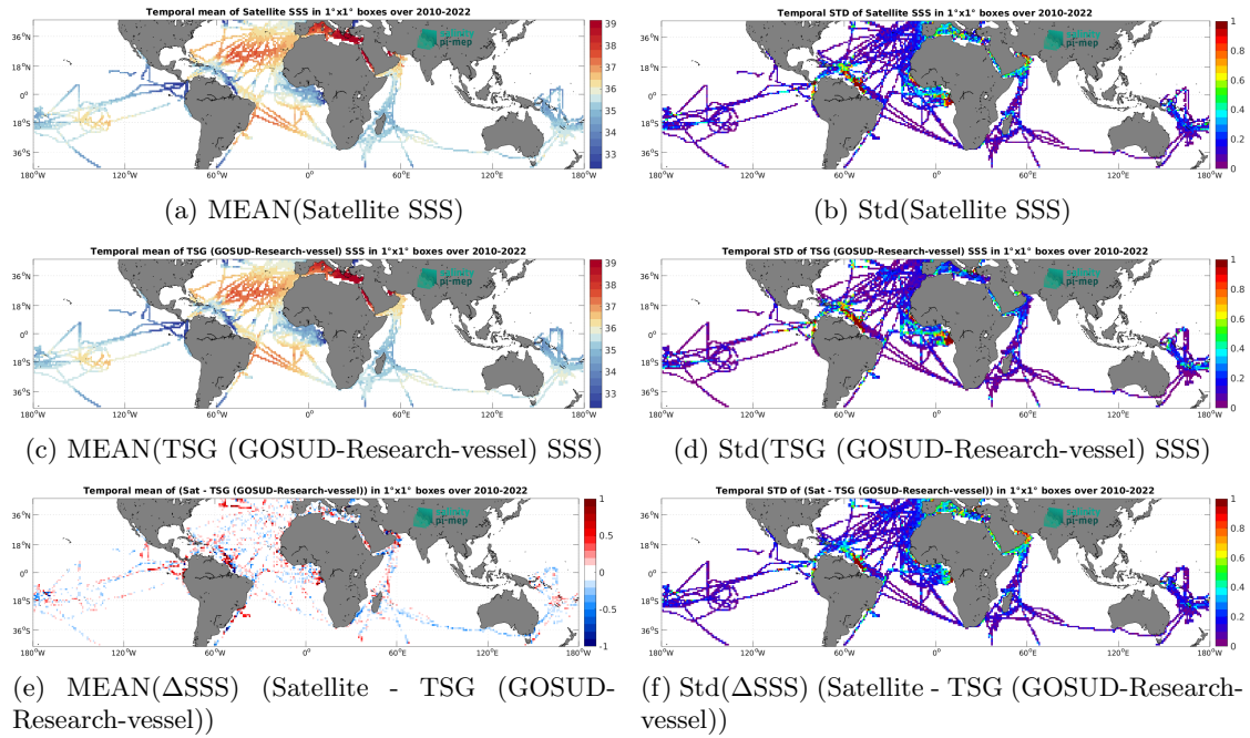
Figure 7: Temporal mean (left) and Std (right) of SSS from SMOS SSS L4 OI v346 - Weekly (CMEMS-CATDS-LOPS) (top), TSG (GOSUD-Research-vessel) (middle), and of \Delta SSS (Satellite - TSG (GOSUD-Research-vessel)). Only match-up pairs are used to generate these maps.
