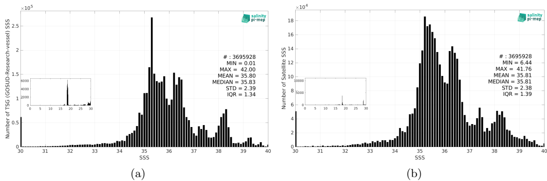
Figure 3: Histograms of SSS from TSG (GOSUD-Research-vessel) (a) and SMOS SSS L4 OI v346 - Weekly (CMEMS-CATDS-LOPS) (b) considering all match-up pairs per bins of 0.1 over the Mid-Low Latitudes 45N-45S Pi-MEP region and for the full satellite product period.
