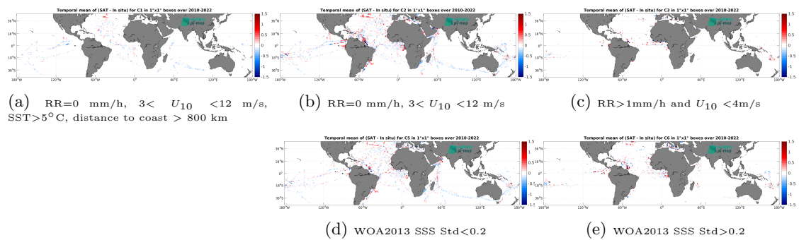
Figure 14: Temporal mean gridded over spatial boxes of size 1^\circ \times 1^\circ of \Delta\text{SSS} (SMOS SSS L4 OI v346 - Weekly (CMEMS-CATDS-LOPS) - TSG (GOSUD-Research-vessel)) for 5 different subdatasets corresponding to: RR=0 mm/h, 3 < U_{10} < 12 m/s, SST > 5°C, distance to coast > 800 km (a), RR=0 mm/h, 3 < U_{10} < 12 m/s (b), RR > 1mm/h and U_{10} < 4 m/s (c), WOA2013 SSS Std < 0.2 (d), WOA2013 SSS Std > 0.2 (e).
