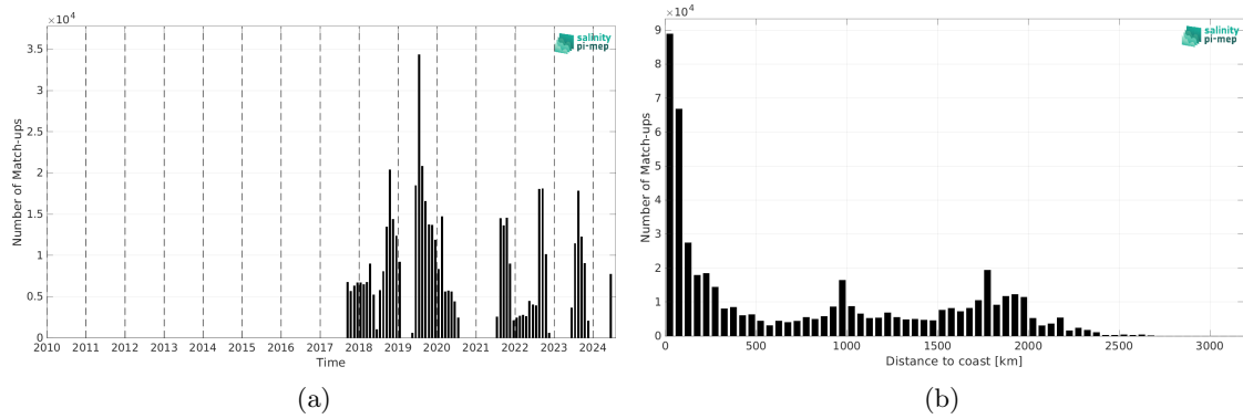
Figure 2: Number of match-ups between Saildrone and SMOS SSS L4 OI v346 - Weekly (CMEMS-CATDS-LOPS) SSS as a function of time (a) and as function of the distance to coast (b) over the Mid-Low Latitudes 45N-45S Pi-MEP region and for the full satellite product period.
