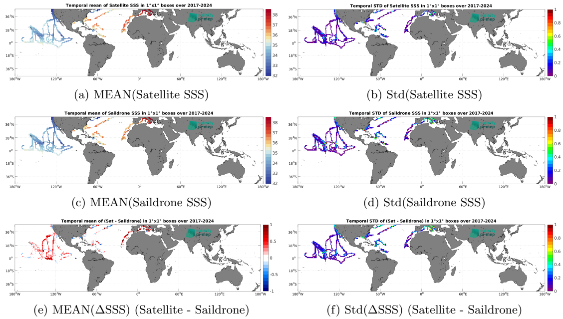
Figure 7: Temporal mean (left) and Std (right) of SSS from SMOS SSS L4 OI v346 - Weekly (CMEMS-CATDS-LOPS) (top), Saildrone (middle), and of \Delta SSS (Satellite - Saildrone). Only match-up pairs are used to generate these maps.
