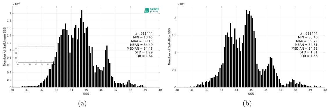
Figure 3: Histograms of SSS from Saildrone (a) and SMOS SSS L4 OI v346 - Weekly (CMEMS-CATDS-LOPS) (b) considering all match-up pairs per bins of 0.1 over the Mid-Low Latitudes 45N-45S Pi-MEP region and for the full satellite product period.
