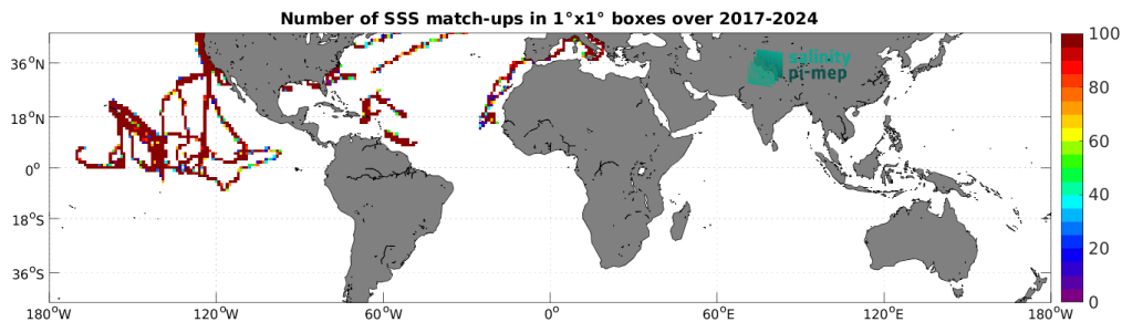
Figure 5: Number of SSS match-ups between Saildrone SSS and the SMOS SSS L4 OI v346 - Weekly (CMEMS-CATDS-LOPS) SSS product for the Mid-Low Latitudes 45N-45S Pi-MEP region over 1^\circ \times 1^\circ boxes and for the full satellite product period.
