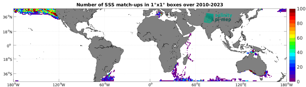
Figure 5: Number of SSS match-ups between Marine mammals SSS and the SMOS SSS L4 OI v346 - Weekly (CMEMS-CATDS-LOPS) SSS product for the Mid-Low Latitudes 45N-45S Pi-MEP region over 1^\circ \times 1^\circ boxes and for the full satellite product period.
