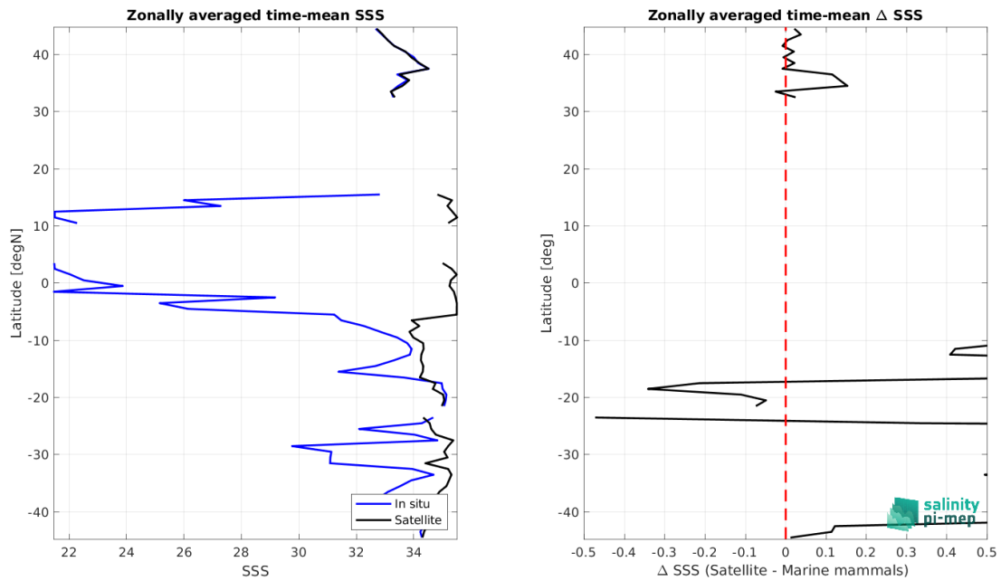
Figure 9: Left panel: Zonal mean SSS from SMOS SSS L4 OI v346 - Weekly (CMEMS-CATDS-LOPS) satellite product (black) and from Marine mammals (blue). Right panel: Zonal mean of \Delta SSS (Satellite - Marine mammals) for all the collected Pi-MEP match-up pairs estimated over the full satellite product period.
