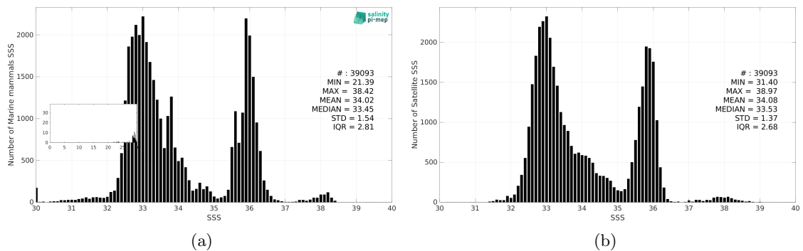
Figure 3: Histograms of SSS from Marine mammals (a) and SMOS SSS L4 OI v346 - Weekly (CMEMS-CATDS-LOPS) (b) considering all match-up pairs per bins of 0.1 over the Mid-Low Latitudes 45N-45S Pi-MEP region and for the full satellite product period.
