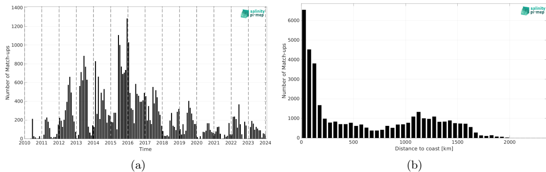
Figure 2: Number of match-ups between Marine mammals and SMOS SSS L4 OI v346 - Weekly (CMEMS-CATDS-LOPS) SSS as a function of time (a) and as function of the distance to coast (b) over the Mid-Low Latitudes 45N-45S Pi-MEP region and for the full satellite product period.
