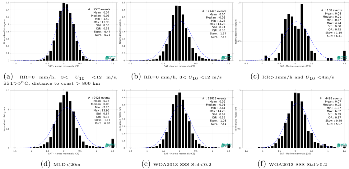
Figure 15: Normalized histogram of \Delta SSS (SMOS SSS L4 OI v346 - Weekly (CMEMS-CATDS-LOPS) - Marine mammals) for 6 different subdatasets corresponding to: RR=0 mm/h, 3 < U_{10} < 12 m/s, SST>5°C, distance to coast > 800 km (a), RR=0 mm/h, 3 < U_{10} < 12 m/s (b), RR>1mm/h and U_{10} < 4 m/s (c), MLD<20m (d), WOA2013 SSS Std<0.2 (e), WOA2013 SSS Std>0.2 (f).
