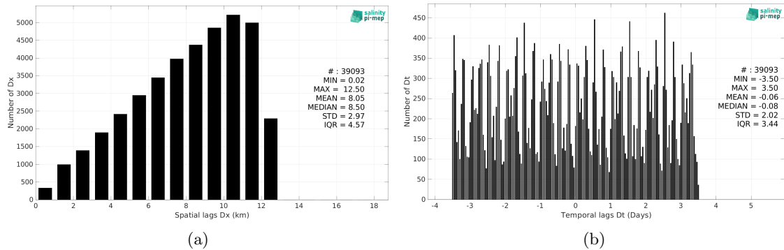
Figure 6: Histograms of the spatial (a) and temporal (b) lags between the location/time of the Marine mammals measurement and the date of the corresponding SMOS SSS L4 OI v346 - Weekly (CMEMS-CATDS-LOPS) SSS pixel.
