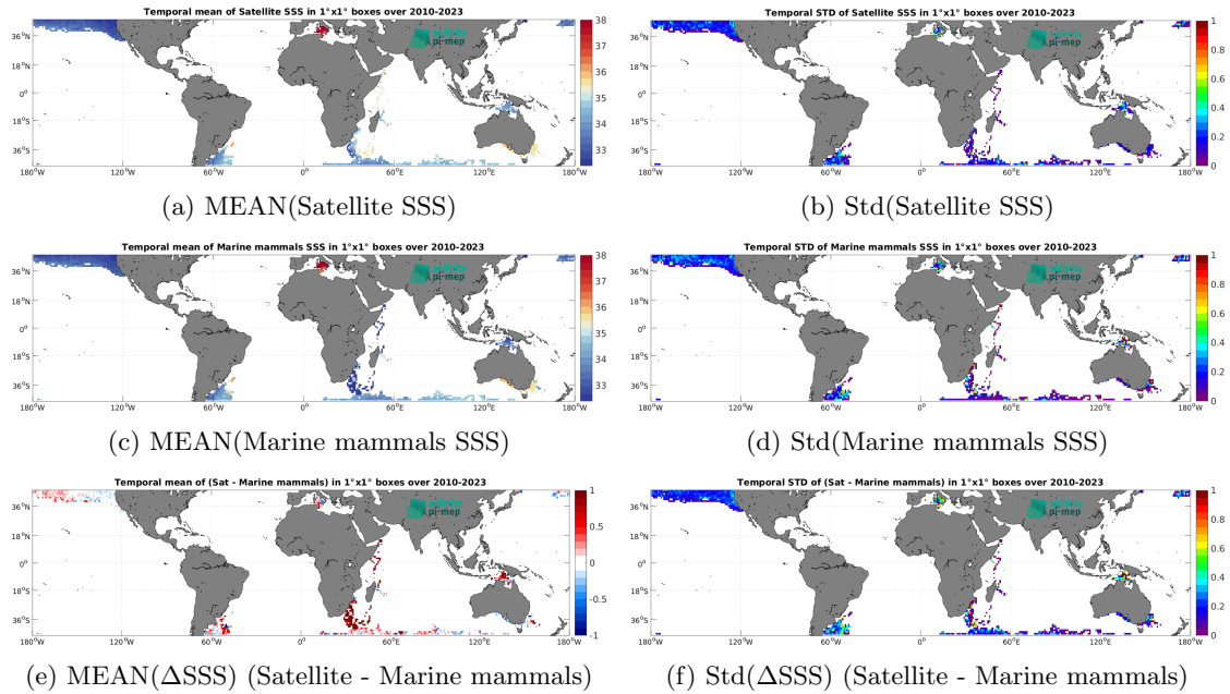
Figure 7: Temporal mean (left) and Std (right) of SSS from SMOS SSS L4 OI v346 - Weekly (CMEMS-CATDS-LOPS) (top), Marine mammals (middle), and of \Delta SSS (Satellite - Marine mammals). Only match-up pairs are used to generate these maps.
