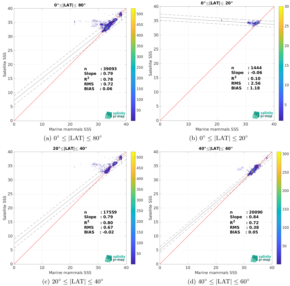
Figure 10: Contour maps of the concentration of SMOS SSS L4 OI v346 - Weekly (CMEMS-CATDS-LOPS) SSS (y-axis) versus Marine mammals SSS (x-axis) at match-up pairs for different latitude bands. For each plot, the red line shows x=y . The black thin and dashed lines indicate a linear fit through the data cloud and the \pm 95\% confidence levels, respectively. The number match-up pairs n , the slope and R^2 coefficient of the linear fit, the root mean square (RMS) and the mean bias between satellite and in situ data are indicated for each latitude band in each plots.
