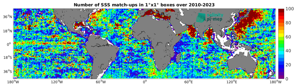
Figure 5: Number of SSS match-ups between Argo SSS and the SMOS SSS L4 OI v346 - Weekly (CMEMS-CATDS-LOPS) SSS product for the Mid-Low Latitudes 45N-45S Pi-MEP region over 1^\circ \times 1^\circ boxes and for the full satellite product period.
