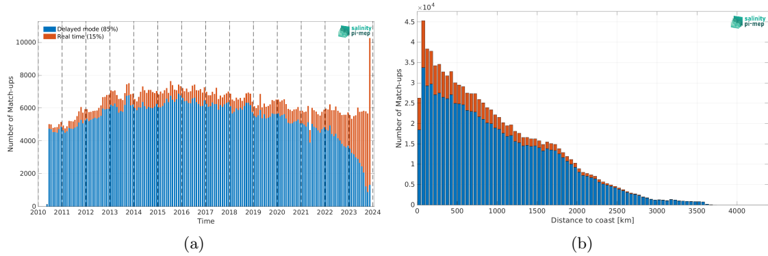
Figure 2: Number of match-ups between Argo and SMOS SSS L4 OI v346 - Weekly (CMEMS-CATDS-LOPS) SSS as a function of time (a) and as function of the distance to coast (b) over the Mid-Low Latitudes 45N-45S Pi-MEP region and for the full satellite product period.
