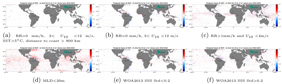
Figure 14: Temporal mean gridded over spatial boxes of size 1^\circ \times 1^\circ of \Delta SSS (SMOS SSS L4 OI v346 - Weekly (CMEMS-CATDS-LOPS) - Argo) for 6 different subdatasets corresponding to:RR=0 mm/h, 3 < U_{10} < 12 m/s, SST>5°C, distance to coast > 800 km (a), RR=0 mm/h, 3 < U_{10} < 12 m/s (b), RR>1mm/h and U_{10} < 4 m/s (c),MLD<20m (d),WOA2013 SSS Std<0.2 (e),WOA2013 SSS Std>0.2 (f).
