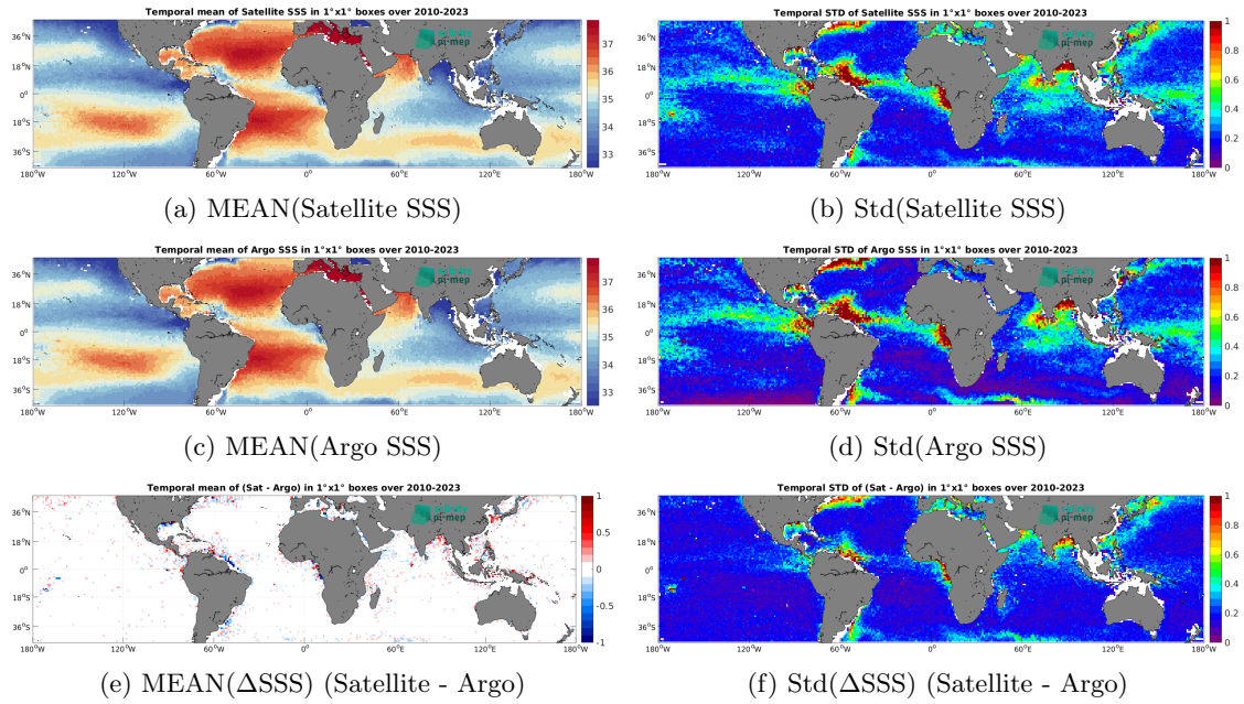
Figure 7: Temporal mean (left) and Std (right) of SSS from SMOS SSS L4 OI v346 - Weekly (CMEMS-CATDS-LOPS) (top), Argo (middle), and of \Delta SSS (Satellite - Argo). Only match-up pairs are used to generate these maps.
