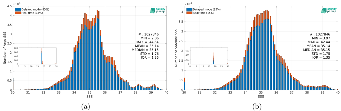
Figure 3: Histograms of SSS from Argo (a) and SMOS SSS L4 OI v346 - Weekly (CMEMS-CATDS-LOPS) (b) considering all match-up pairs per bins of 0.1 over the Mid-Low Latitudes 45N-45S Pi-MEP region and for the full satellite product period.
