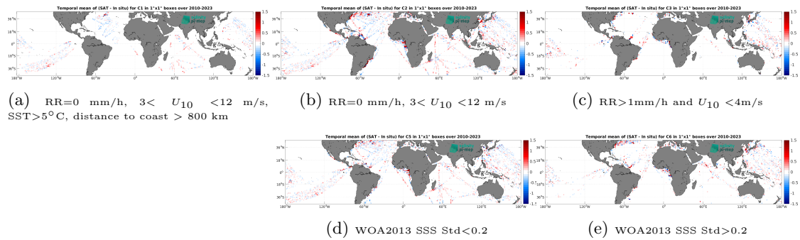
Figure 12: Temporal mean gridded over spatial boxes of size 1^\circ \times 1^\circ of \Delta\text{SSS} (SMOS SSS L4 OI v342 - Weekly (CMEMS-CATDS-LOPS) - TSG (LEGOS-DM)) for 5 different subdatasets corresponding to:RR=0 mm/h, 3 < U_{10} < 12 m/s, SST >5^\circ\text{C} , distance to coast > 800 km (a), RR=0 mm/h, 3 < U_{10} < 12 m/s (b), RR >1 mm/h and U_{10} < 4 m/s (c), WOA2013 SSS Std <0.2 (d), WOA2013 SSS Std >0.2 (e).
