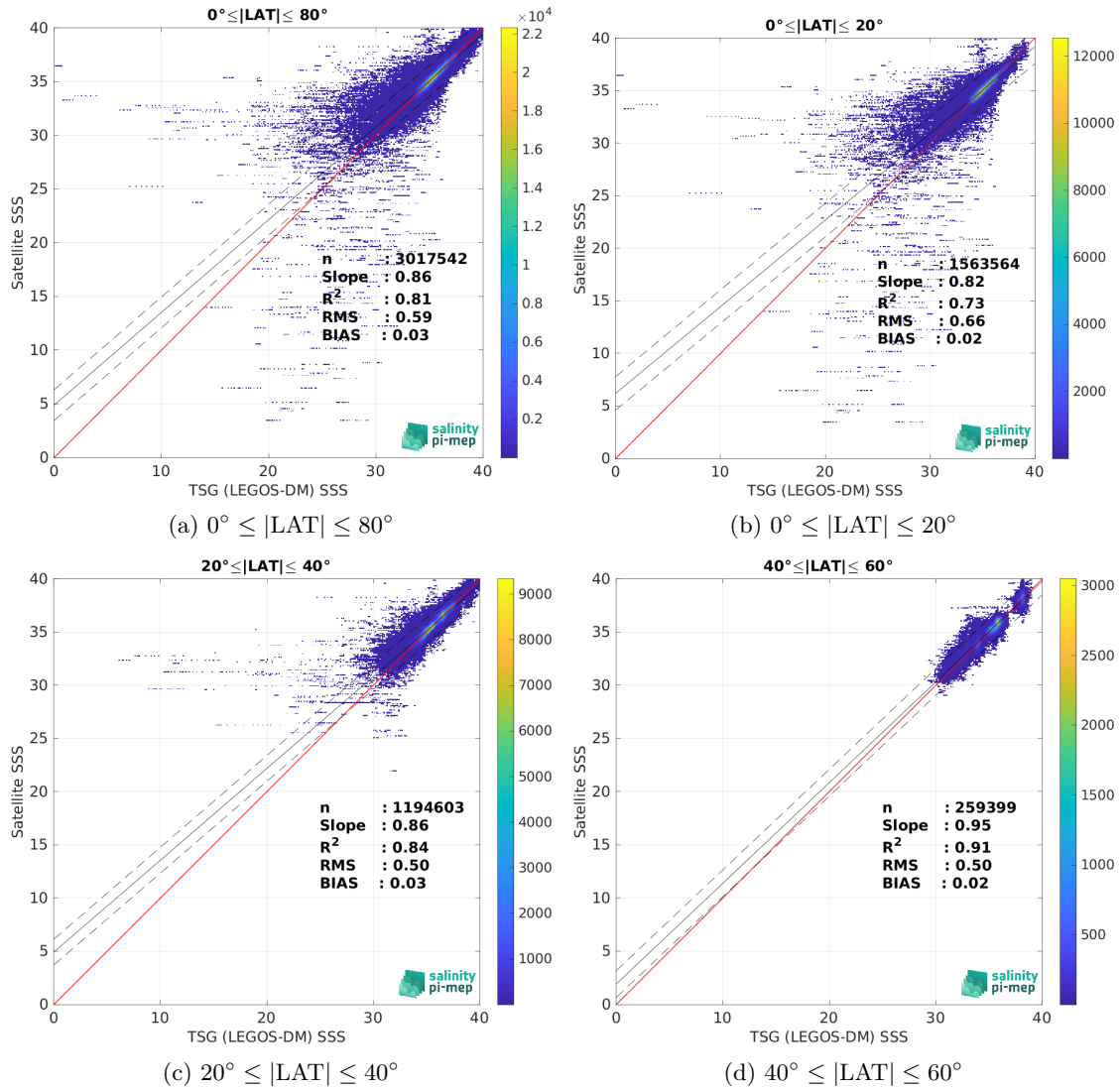
Figure 9: Contour maps of the concentration of SMOS SSS L4 OI v342 - Weekly (CMEMS-CATDS-LOPS) SSS (y-axis) versus TSG (LEGOS-DM) SSS (x-axis) at match-up pairs for different latitude bands. For each plot, the red line shows x=y . The black thin and dashed lines indicate a linear fit through the data cloud and the \pm 95\% confidence levels, respectively. The number match-up pairs n , the slope and R^2 coefficient of the linear fit, the root mean square (RMS) and the mean bias between satellite and in situ data are indicated for each latitude band in each plots.
