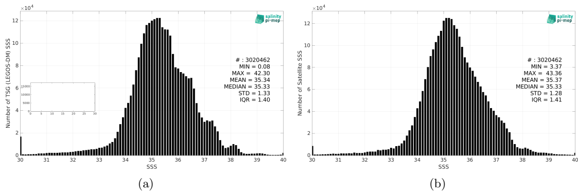
Figure 2: Histograms of SSS from TSG (LEGOS-DM) (a) and SMOS SSS L4 OI v342 - Weekly (CMEMS-CATDS-LOPS) (b) considering all match-up pairs per bins of 0.1 over the Mid-Low Latitudes 45N-45S Pi-MEP region and for the full satellite product period.
