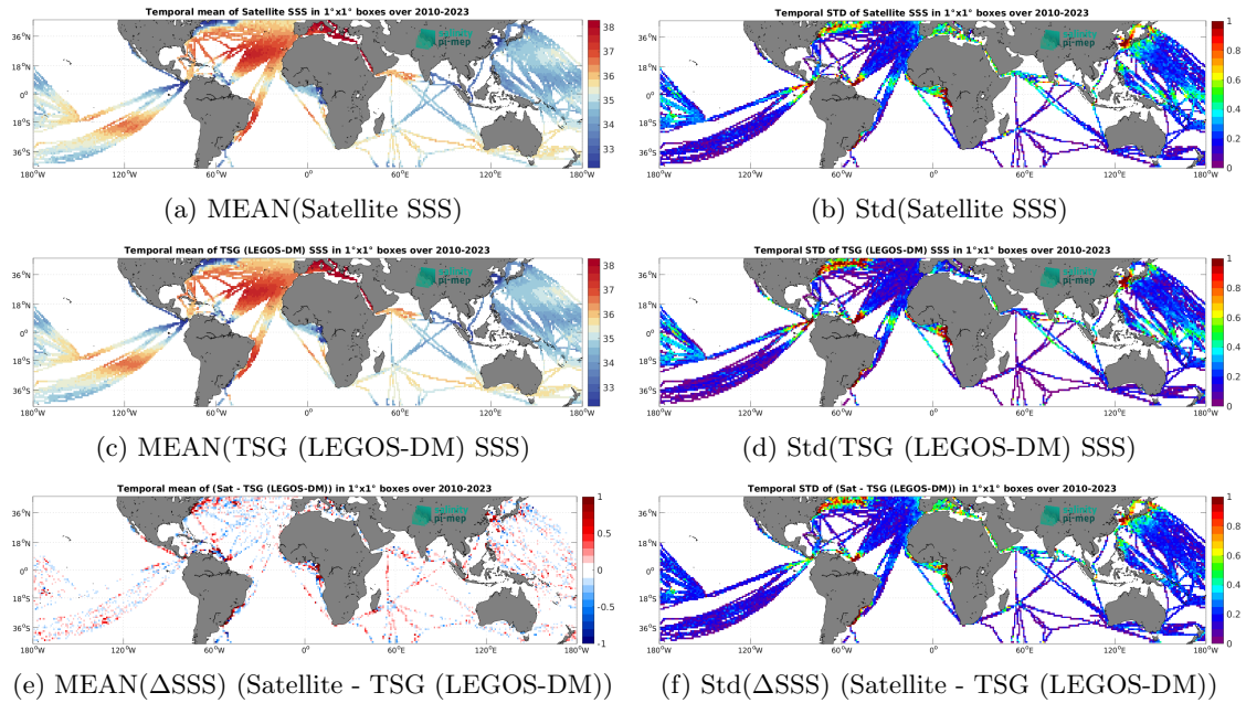
Figure 6: Temporal mean (left) and Std (right) of SSS from SMOS SSS L4 OI v342 - Weekly (CMEMS-CATDS-LOPS) (top), TSG (LEGOS-DM) (middle), and of \Delta SSS (Satellite - TSG (LEGOS-DM)). Only match-up pairs are used to generate these maps.
