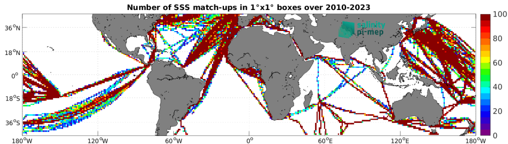
Figure 4: Number of SSS match-ups between TSG (LEGOS-DM) SSS and the SMOS SSS L4 OI v342 - Weekly (CMEMS-CATDS-LOPS) SSS product for the Mid-Low Latitudes 45N-45S Pi-MEP region over 1^\circ \times 1^\circ boxes and for the full satellite product period.
