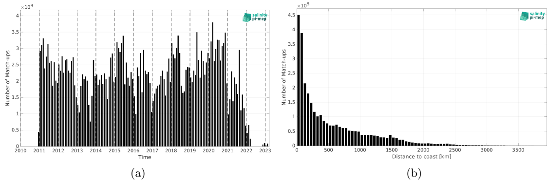
Figure 1: Number of match-ups between TSG (LEGOS-DM) and SMOS SSS L4 OI v342 - Weekly (CMEMS-CATDS-LOPS) SSS as a function of time (a) and as function of the distance to coast (b) over the Mid-Low Latitudes 45N-45S Pi-MEP region and for the full satellite product period.
