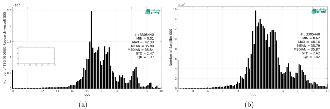
Figure 2: Histograms of SSS from TSG (GOSUD-Research-vessel) (a) and SMOS SSS L4 OI v342 - Weekly (CMEMS-CATDS-LOPS) (b) considering all match-up pairs per bins of 0.1 over the Mid-Low Latitudes 45N-45S Pi-MEP region and for the full satellite product period.
