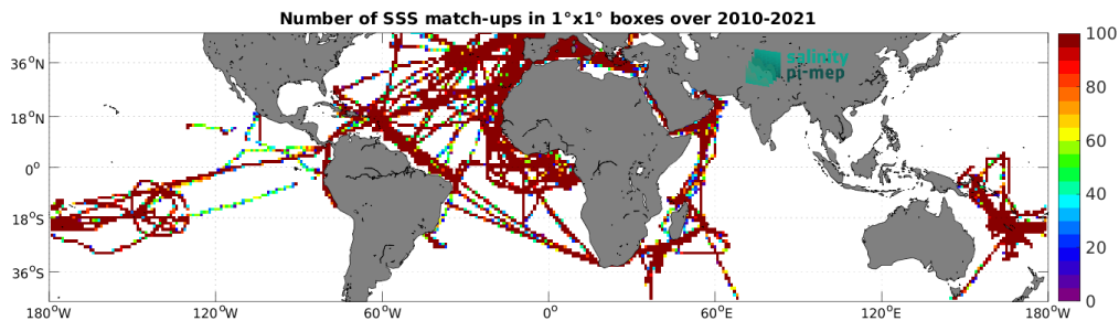
Figure 4: Number of SSS match-ups between TSG (GOSUD-Research-vessel) SSS and the SMOS SSS L4 OI v342 - Weekly (CMEMS-CATDS-LOPS) SSS product for the Mid-Low Latitudes 45N-45S Pi-MEP region over 1^\circ \times 1^\circ boxes and for the full satellite product period.
