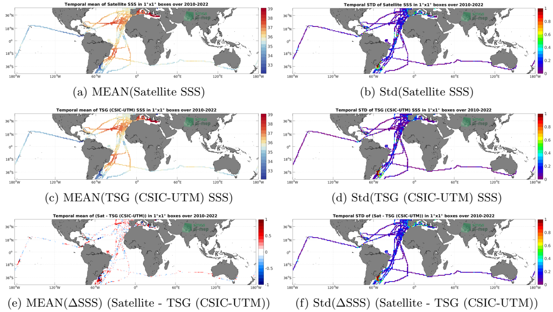
Figure 6: Temporal mean (left) and Std (right) of SSS from SMOS SSS L4 OI v342 - Weekly (CMEMS-CATDS-LOPS) (top), TSG (CSIC-UTM) (middle), and of \Delta SSS (Satellite - TSG (CSIC-UTM)). Only match-up pairs are used to generate these maps.
