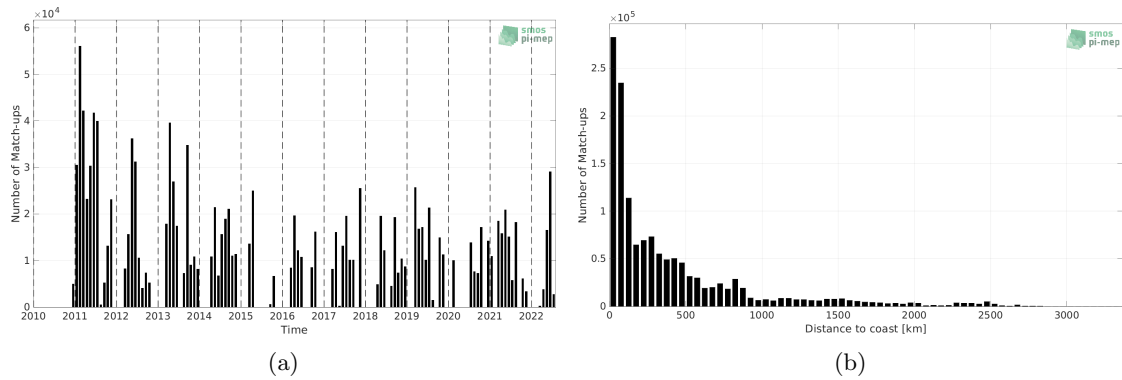
Figure 1: Number of match-ups between TSG (CSIC-UTM) and SMOS SSS L4 OI v342 - Weekly (CMEMS-CATDS-LOPS) SSS as a function of time (a) and as function of the distance to coast (b) over the Mid-Low Latitudes 45N-45S Pi-MEP region and for the full satellite product period.
