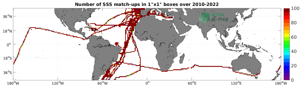
Figure 4: Number of SSS match-ups between TSG (CSIC-UTM) SSS and the SMOS SSS L4 OI v342 - Weekly (CMEMS-CATDS-LOPS) SSS product for the Mid-Low Latitudes 45N-45S Pi-MEP region over 1^\circ \times 1^\circ boxes and for the full satellite product period.
