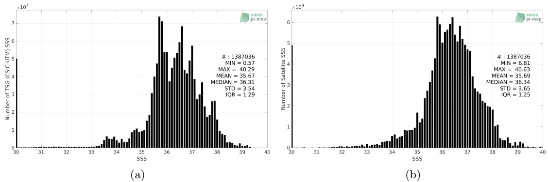
Figure 2: Histograms of SSS from TSG (CSIC-UTM) (a) and SMOS SSS L4 OI v342 - Weekly (CMEMS-CATDS-LOPS) (b) considering all match-up pairs per bins of 0.1 over the Mid-Low Latitudes 45N-45S Pi-MEP region and for the full satellite product period.
