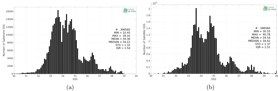
Figure 2: Histograms of SSS from Saildrone (a) and SMOS SSS L4 OI v342 - Weekly (CMEMS-CATDS-LOPS) (b) considering all match-up pairs per bins of 0.1 over the Mid-Low Latitudes 45N-45S Pi-MEP region and for the full satellite product period.
