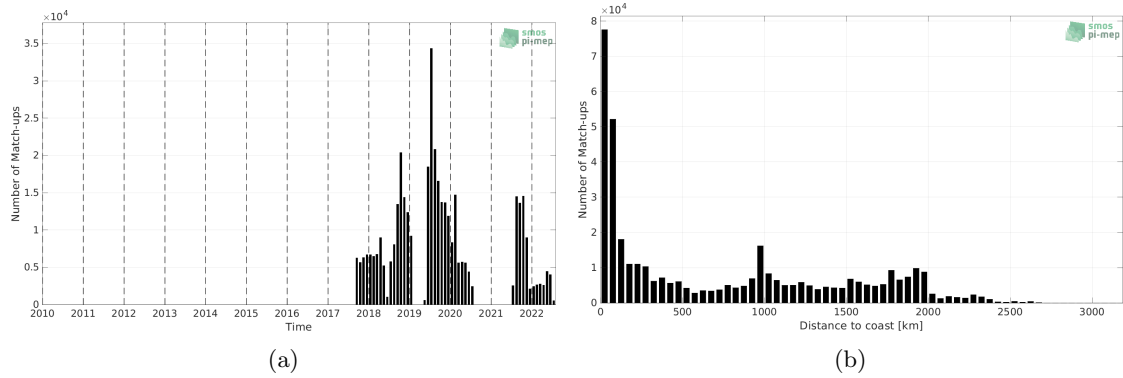
Figure 1: Number of match-ups between Saildrone and SMOS SSS L4 OI v342 - Weekly (CMEMS-CATDS-LOPS) SSS as a function of time (a) and as function of the distance to coast (b) over the Mid-Low Latitudes 45N-45S Pi-MEP region and for the full satellite product period.
