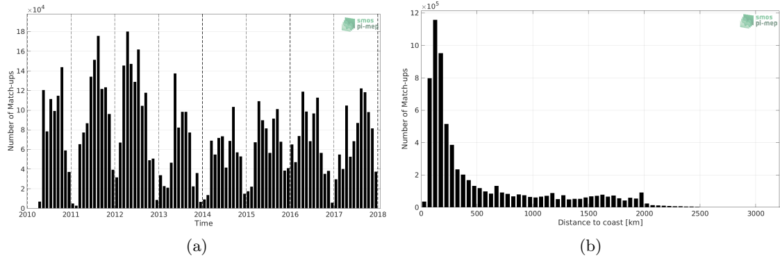
Figure 1: Number of match-ups between TSG (SAMOS) and SMOS L4 v2 Weekly (CATDS-CECOS-IFREMER) SSS as a function of time (a) and as function of the distance to coast (b) over the Mid-Low Latitudes 45N-45S Pi-MEP region and for the full satellite product period.
