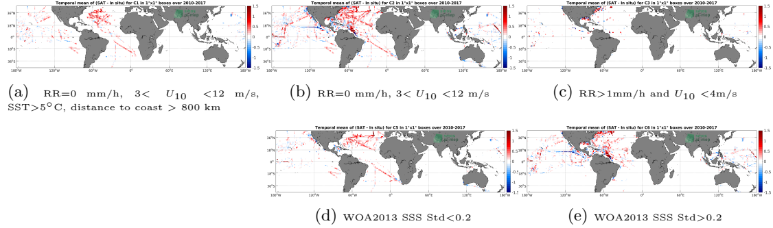
Figure 12: Temporal mean gridded over spatial boxes of size 1^\circ \times 1^\circ of \Delta SSS (SMOS L4 v2 Weekly (CATDS-CECOS-IFREMER) - TSG (SAMOS)) for 5 different subdatasets corresponding to: RR=0 mm/h, 3 < U_{10} < 12 m/s, SST > 5^\circ C , distance to coast > 800 km (a), RR=0 mm/h, 3 < U_{10} < 12 m/s (b), RR > 1 mm/h and U_{10} < 4 m/s (c), WOA2013 SSS Std < 0.2 (d), WOA2013 SSS Std > 0.2 (e).
