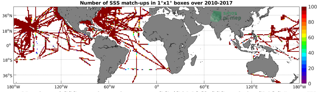
Figure 4: Number of SSS match-ups between TSG (SAMOS) SSS and the SMOS L4 v2 Weekly (CATDS-CECOS-IFREMER) SSS product for the Mid-Low Latitudes 45N-45S Pi-MEP region over 1°x1° boxes and for the full satellite product period.
