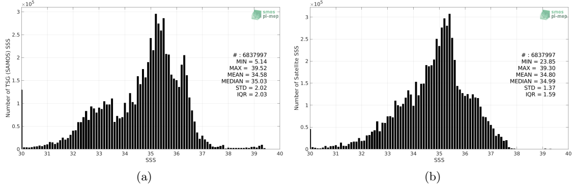
Figure 2: Histograms of SSS from TSG (SAMOS) (a) and SMOS L4 v2 Weekly (CATDS-CECOS-IFREMER) (b) considering all match-up pairs per bins of 0.1 over the Mid-Low Latitudes 45N-45S Pi-MEP region and for the full satellite product period.
