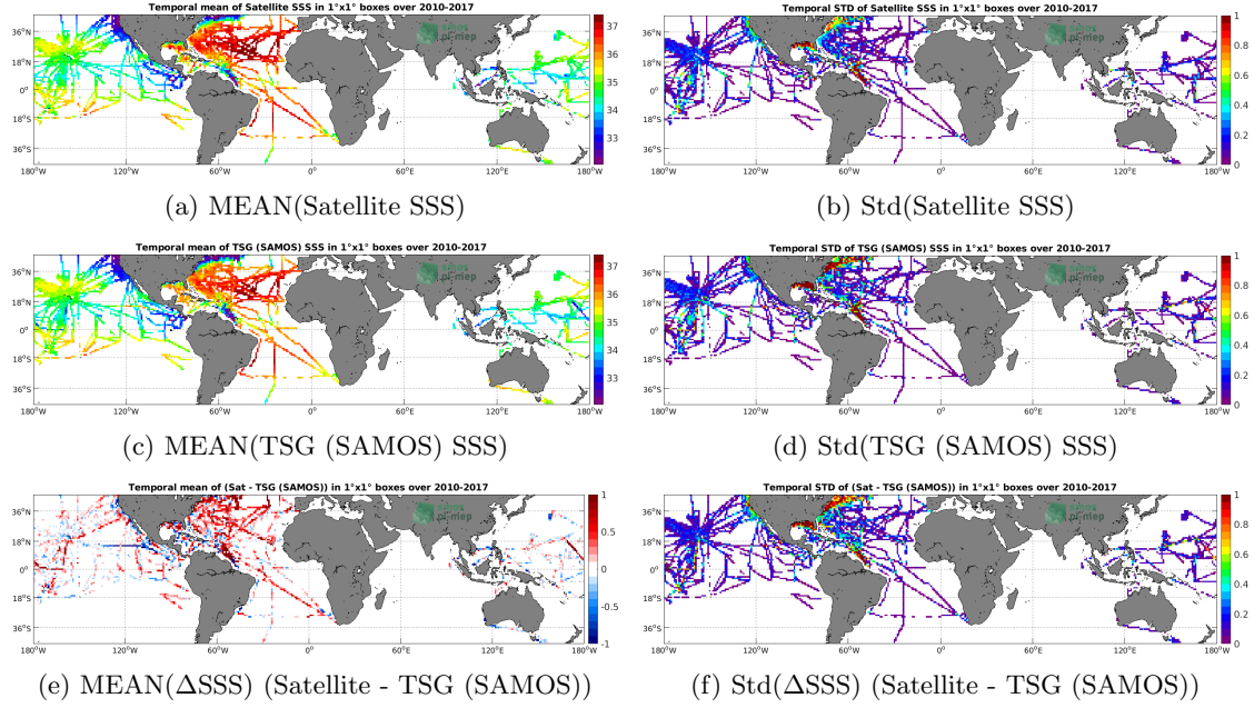
Figure 6: Temporal mean (left) and Std (right) of SSS from SMOS L4 v2 Weekly (CATDS-CECOS-IFREMER) (top), TSG (SAMOS) (middle), and of \Delta SSS (Satellite - TSG (SAMOS)). Only match-up pairs are used to generate these maps.
