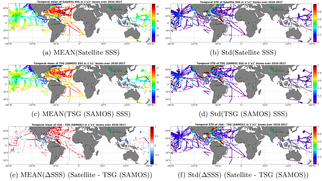
Figure 6: Temporal mean (left) and Std (right) of SSS from SMOS L4 v2 Weekly (CATDS-CECOS-IFREMER) (top), TSG (SAMOS) (middle), and of \Delta SSS (Satellite - TSG (SAMOS)). Only match-up pairs are used to generate these maps.
