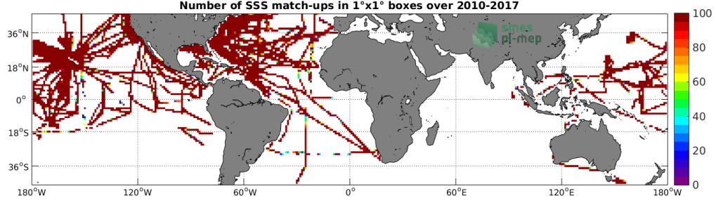
Figure 4: Number of SSS match-ups between TSG-SAMOS SSS and the SMOS-L4-CATDS-CECOS-IFREMER-V2-WEEKLY-0.5DEG SSS product for the Mid-Low Latitudes 45N-45S Pi-MEP region over 1°x1° boxes and for the full satellite product period.
