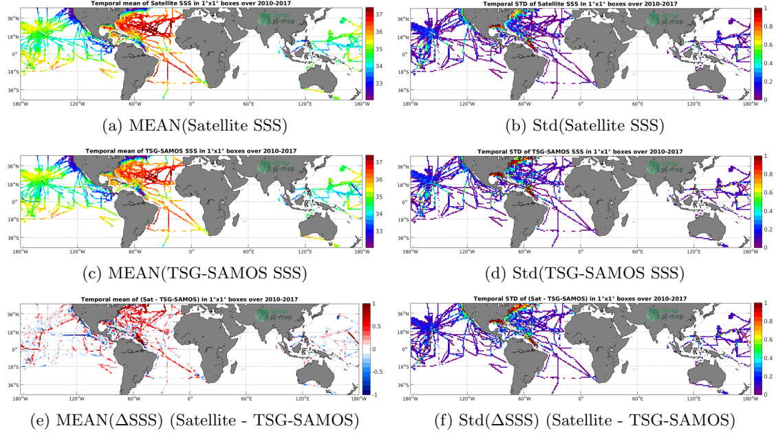
Figure 6: Temporal mean (left) and Std (right) of SSS from SMOS-L4-CATDS-CECOS-IFREMER-V2-WEEKLY-0.5DEG (top), TSG-SAMOS (middle), and of \Delta SSS (Satellite - TSG-SAMOS). Only match-up pairs are used to generate these maps.
