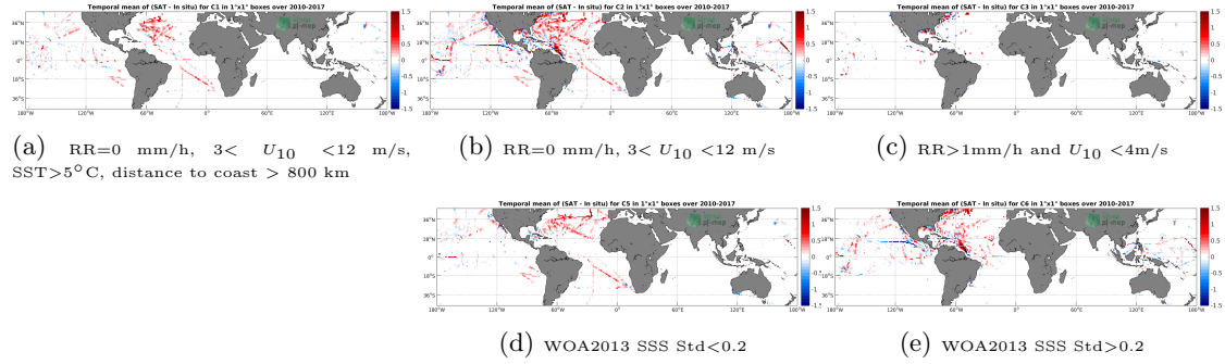
Figure 12: Temporal mean gridded over spatial boxes of size 1^\circ \times 1^\circ of \Delta SSS (SMOS-L4-CATDS-CECOS-IFREMER-V2-WEEKLY-0.5DEG - TSG-SAMOS) for 5 different subdatasets corresponding to: RR=0 mm/h, 3 < U_{10} < 12 m/s, SST > 5^\circ C , distance to coast > 800 km (a), RR=0 mm/h, 3 < U_{10} < 12 m/s (b), RR > 1 mm/h and U_{10} < 4 m/s (c), WOA2013 SSS Std < 0.2 (d), WOA2013 SSS Std > 0.2 (e).
