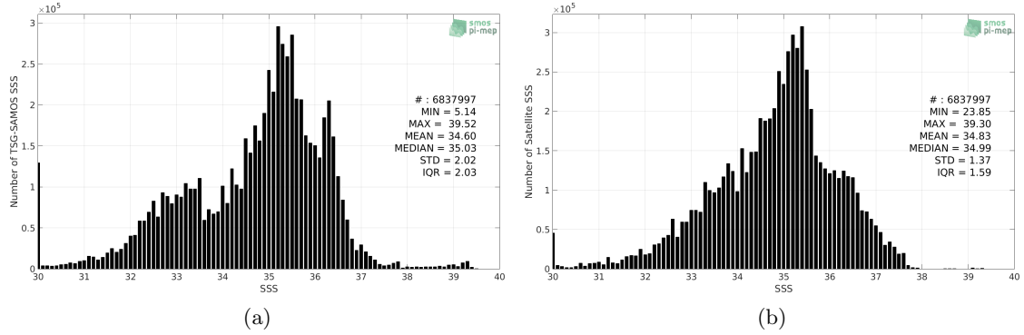
Figure 2: Histograms of SSS from TSG-SAMOS (a) and SMOS-L4-CATDS-CECOS-IFREMER-V2-WEEKLY-0.5DEG (b) considering all match-up pairs per bins of 0.1 over the Mid-Low Latitudes 45N-45S Pi-MEP region and for the full satellite product period.
