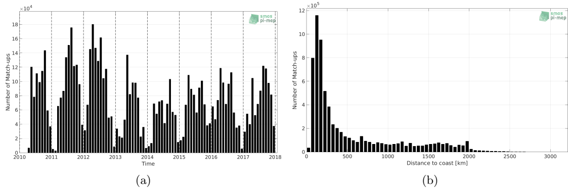
Figure 1: Number of match-ups between TSG-SAMOS and SMOS-L4-CATDS-CECOS-IFREMER-V2-WEEKLY-0.5DEG SSS as a function of time (a) and as function of the distance to coast (b) over the Mid-Low Latitudes 45N-45S Pi-MEP region and for the full satellite product period.
