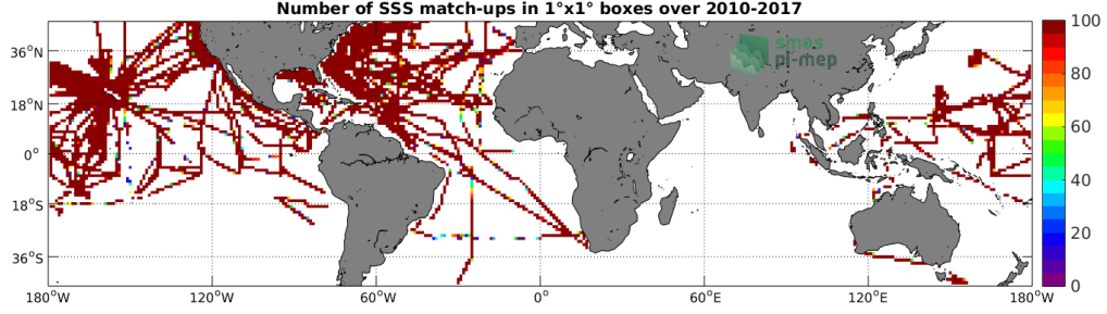
Figure 4: Number of SSS match-ups between TSG-SAMOS SSS and the SMOS-L4-CATDS-CECOS-IFREMER-V2-WEEKLY-0.5DEG SSS product for the Mid-Low Latitudes 45N-45S Pi-MEP region over 1^\circ \times 1^\circ boxes and for the full satellite product period.
