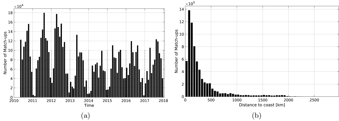
Figure 1: Number of match-ups between TSG-SAMOS and SMOS-L4-CATDS-CECOS-IFREMER-V2-WEEKLY-0.5DEG SSS as a function of time (a) and as function of the distance to coast (b) over the Mid-Low Latitudes 45N-45S Pi-MEP region and for the full satellite product period.
