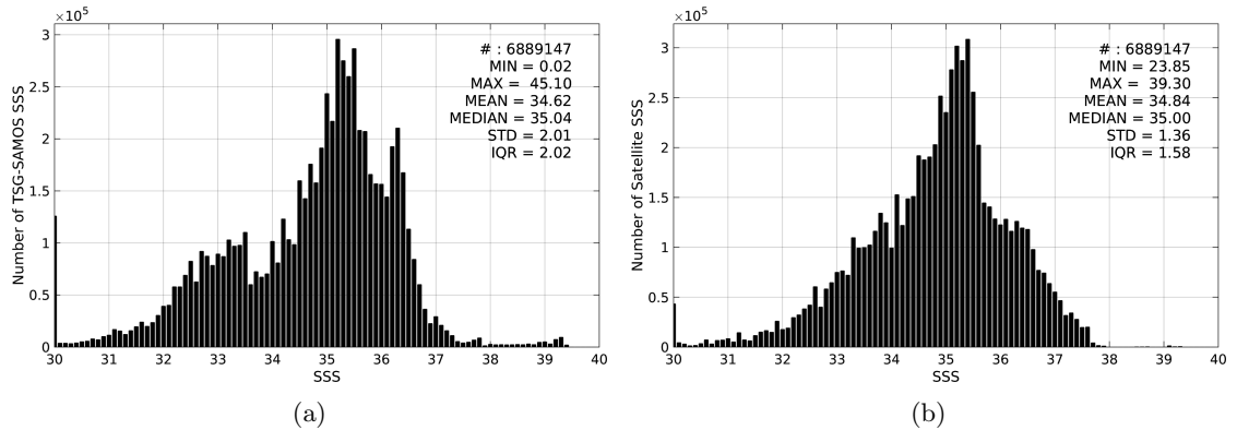
Figure 2: Histograms of SSS from TSG-SAMOS (a) and SMOS-L4-CATDS-CECOS-IFREMER-V2-WEEKLY-0.5DEG (b) considering all match-up pairs per bins of 0.1 over the Mid-Low Latitudes 45N-45S Pi-MEP region and for the full satellite product period.
