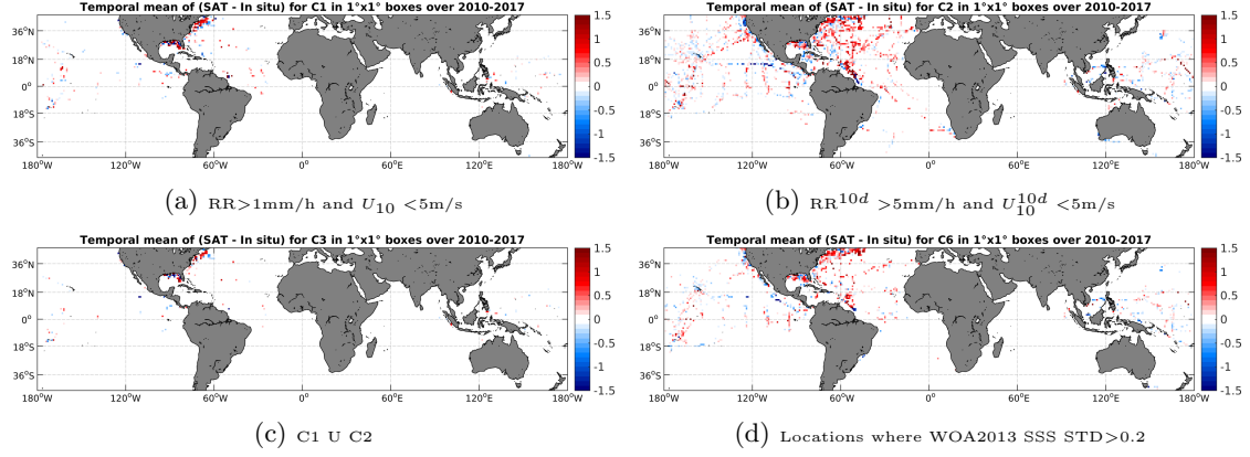
Figure 12: Temporal mean gridded over spatial boxes of size 1^\circ \times 1^\circ of \Delta SSS (SMOS-L4-CATDS-CECOS-IFREMER-V2-WEEKLY-0.5DEG - TSG-SAMOS) for 4 different subdatasets corresponding to: RR > 1\text{mm/h} and U_{10} < 5\text{m/s} (a), RR^{10d} > 5\text{mm/h} and U_{10}^{10d} < 5\text{m/s} (b), C1 U C2 (c), Locations where WOA2013 SSS STD > 0.2 (d).
