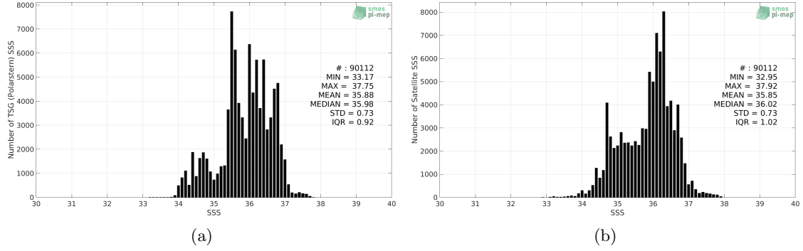
Figure 2: Histograms of SSS from TSG (Polarstern) (a) and SMOS L4 v2 Weekly (CATDS-CECOS-IFREMER) (b) considering all match-up pairs per bins of 0.1 over the Mid-Low Latitudes 45N-45S Pi-MEP region and for the full satellite product period.
