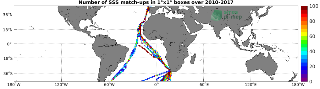
Figure 4: Number of SSS match-ups between TSG (Polarstern) SSS and the SMOS L4 v2 Weekly (CATDS-CECOS-IFREMER) SSS product for the Mid-Low Latitudes 45N-45S Pi-MEP region over 1°x1° boxes and for the full satellite product period.
