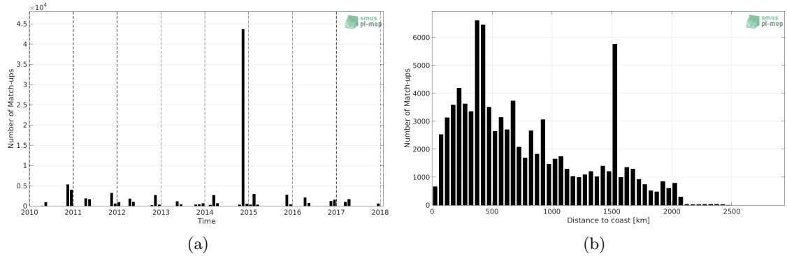
Figure 1: Number of match-ups between TSG (Polarstern) and SMOS L4 v2 Weekly (CATDS-CECOS-IFREMER) SSS as a function of time (a) and as function of the distance to coast (b) over the Mid-Low Latitudes 45N-45S Pi-MEP region and for the full satellite product period.
