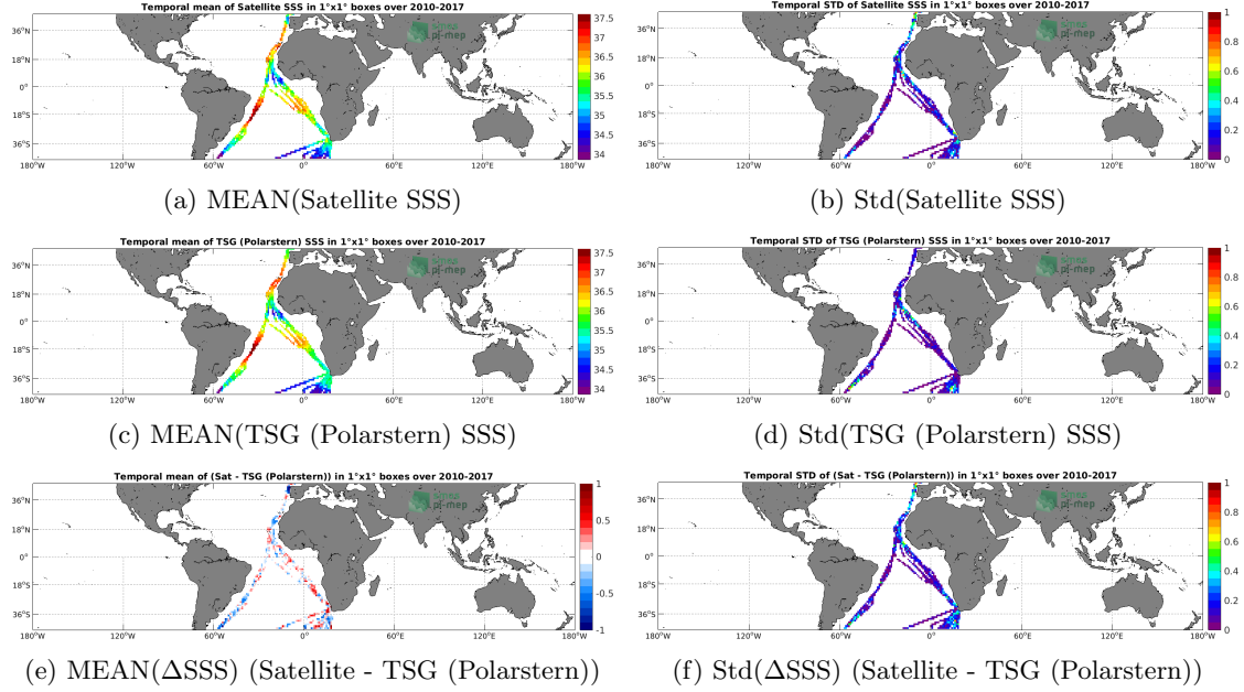
Figure 6: Temporal mean (left) and Std (right) of SSS from SMOS L4 v2 Weekly (CATDS-CECOS-IFREMER) (top), TSG (Polarstern) (middle), and of \Delta SSS (Satellite - TSG (Polarstern)). Only match-up pairs are used to generate these maps.
