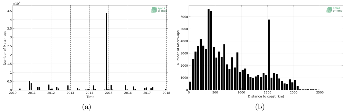
Figure 1: Number of match-ups between TSG-POLARSTERN and SMOS-L4-CATDS-CECOS-IFREMER-V2-WEEKLY-0.5DEG SSS as a function of time (a) and as function of the distance to coast (b) over the Mid-Low Latitudes 45N-45S Pi-MEP region and for the full satellite product period.
