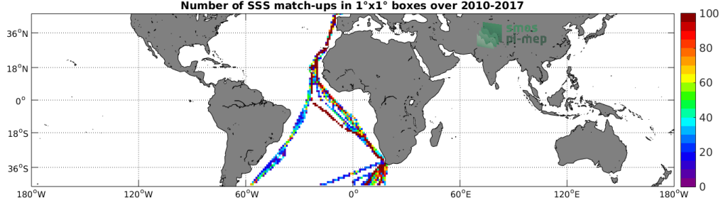
Figure 4: Number of SSS match-ups between TSG-POLARSTERN SSS and the SMOS-L4-CATDS-CECOS-IFREMER-V2-WEEKLY-0.5DEG SSS product for the Mid-Low Latitudes 45N-45S Pi-MEP region over 1^\circ \times 1^\circ boxes and for the full satellite product period.
