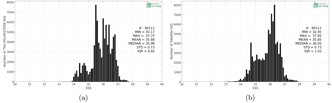
Figure 2: Histograms of SSS from TSG-POLARSTERN (a) and SMOS-L4-CATDS-CECOS-IFREMER-V2-WEEKLY-0.5DEG (b) considering all match-up pairs per bins of 0.1 over the Mid-Low Latitudes 45N-45S Pi-MEP region and for the full satellite product period.
