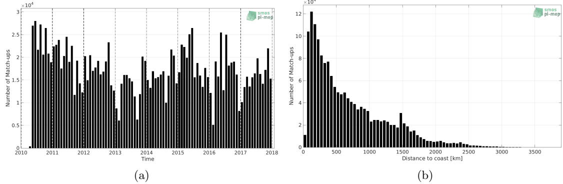
Figure 1: Number of match-ups between TSG (LEGOS-DM) and SMOS L4 v2 Weekly (CATDS-CECOS-IFREMER) SSS as a function of time (a) and as function of the distance to coast (b) over the Mid-Low Latitudes 45N-45S Pi-MEP region and for the full satellite product period.
