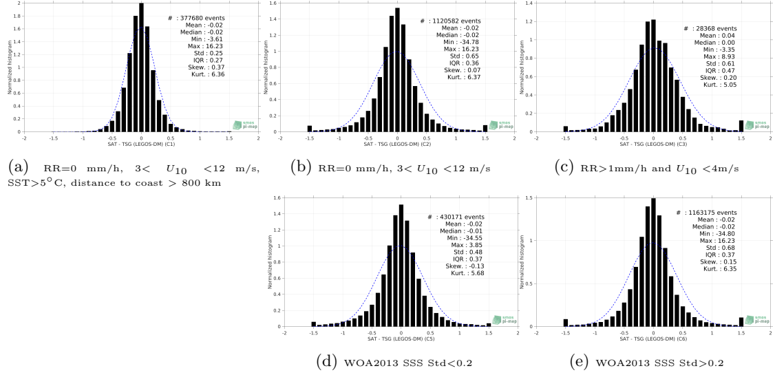
Figure 13: Normalized histogram of \Delta\text{SSS} (SMOS L4 v2 Weekly (CATDS-CECOS-IFREMER) - TSG (LEGOS-DM)) for 5 different subdatasets corresponding to: RR=0 mm/h, 3 < U_{10} < 12 m/s, SST > 5^\circ\text{C} , distance to coast > 800 km (a), RR=0 mm/h, 3 < U_{10} < 12 m/s (b), RR > 1\text{mm/h} and U_{10} < 4\text{m/s} (c), WOA2013 SSS Std < 0.2 (d), WOA2013 SSS Std > 0.2 (e).
