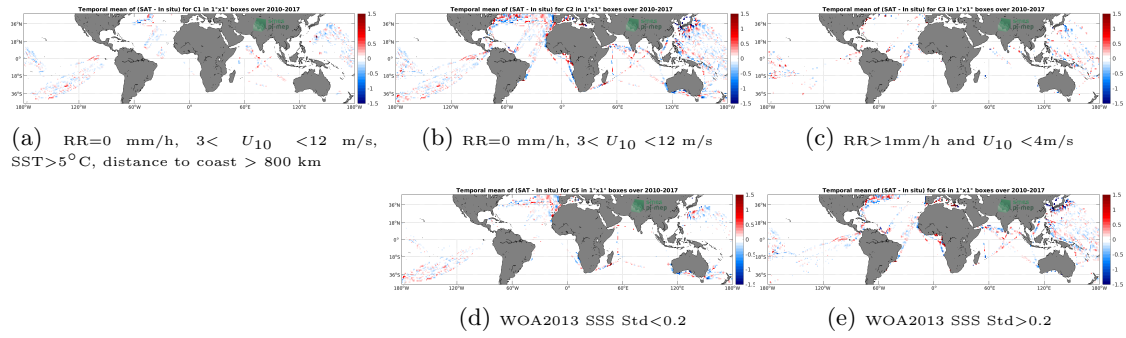
Figure 12: Temporal mean gridded over spatial boxes of size 1^\circ \times 1^\circ of \Delta SSS (SMOS L4 v2 Weekly (CATDS-CECOS-IFREMER) - TSG (LEGOS-DM)) for 5 different subdatasets corresponding to: RR=0 mm/h, 3 < U_{10} < 12 m/s, SST > 5^\circ C , distance to coast > 800 km (a), RR=0 mm/h, 3 < U_{10} < 12 m/s (b), RR > 1 mm/h and U_{10} < 4 m/s (c), WOA2013 SSS Std < 0.2 (d), WOA2013 SSS Std > 0.2 (e).
