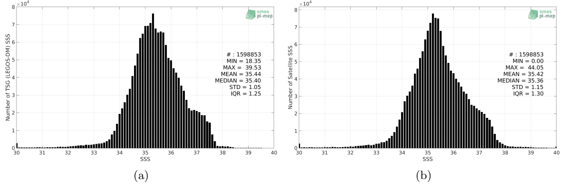
Figure 2: Histograms of SSS from TSG (LEGOS-DM) (a) and SMOS L4 v2 Weekly (CATDS-CECOS-IFREMER) (b) considering all match-up pairs per bins of 0.1 over the Mid-Low Latitudes 45N-45S Pi-MEP region and for the full satellite product period.
