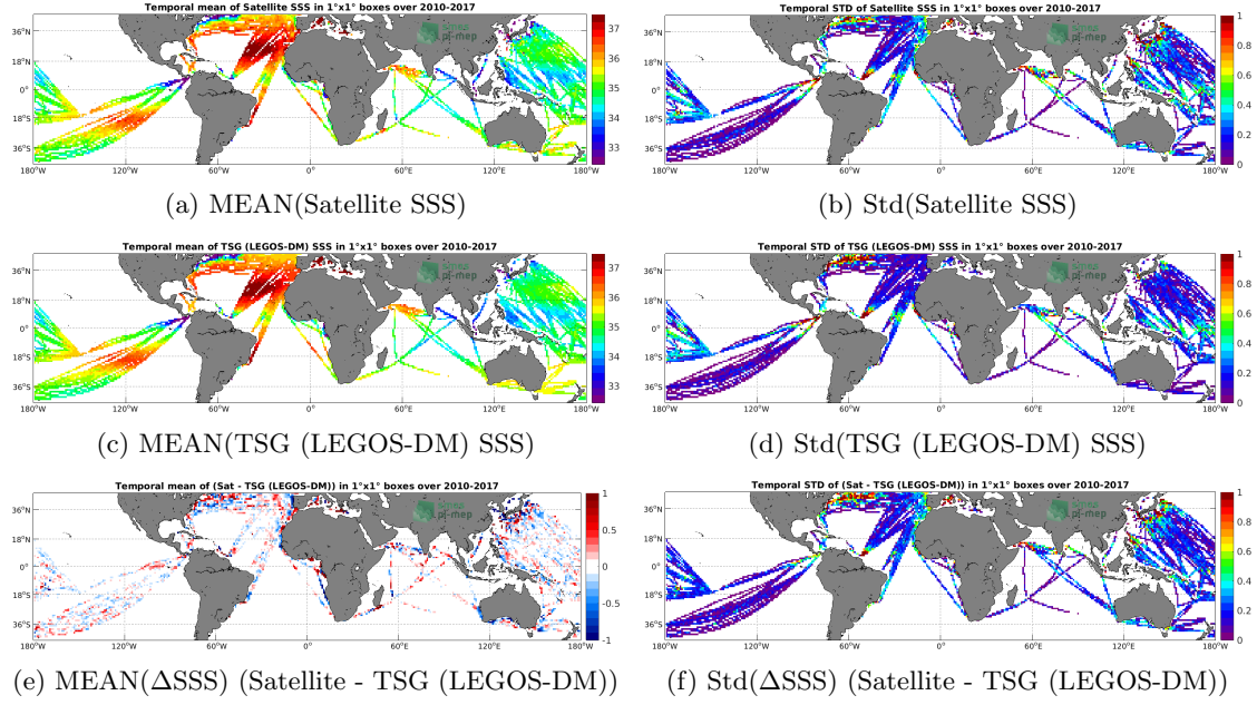
Figure 6: Temporal mean (left) and Std (right) of SSS from SMOS L4 v2 Weekly (CATDS-CECOS-IFREMER) (top), TSG (LEGOS-DM) (middle), and of \Delta SSS (Satellite - TSG (LEGOS-DM)). Only match-up pairs are used to generate these maps.
