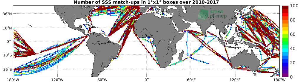
Figure 4: Number of SSS match-ups between TSG (LEGOS-DM) SSS and the SMOS L4 v2 Weekly (CATDS-CECOS-IFREMER) SSS product for the Mid-Low Latitudes 45N-45S Pi-MEP region over 1°x1° boxes and for the full satellite product period.
