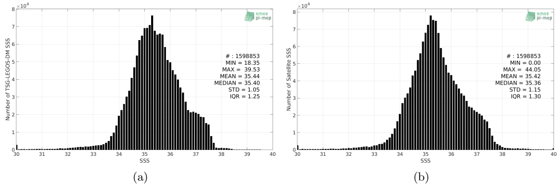
Figure 2: Histograms of SSS from TSG-LEGOS-DM (a) and SMOS-L4-CATDS-CECOS-IFREMER-V2-WEEKLY-0.5DEG (b) considering all match-up pairs per bins of 0.1 over the Mid-Low Latitudes 45N-45S Pi-MEP region and for the full satellite product period.
