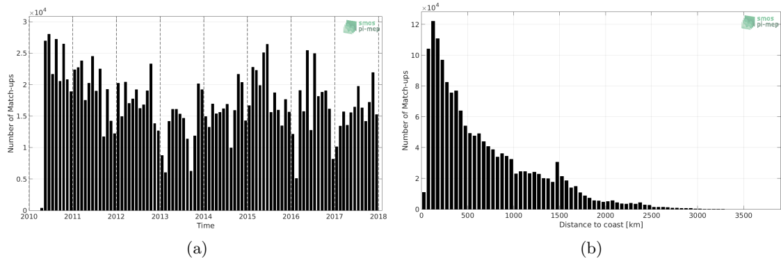
Figure 1: Number of match-ups between TSG-LEGOS-DM and SMOS-L4-CATDS-CECOS-IFREMER-V2-WEEKLY-0.5DEG SSS as a function of time (a) and as function of the distance to coast (b) over the Mid-Low Latitudes 45N-45S Pi-MEP region and for the full satellite product period.
