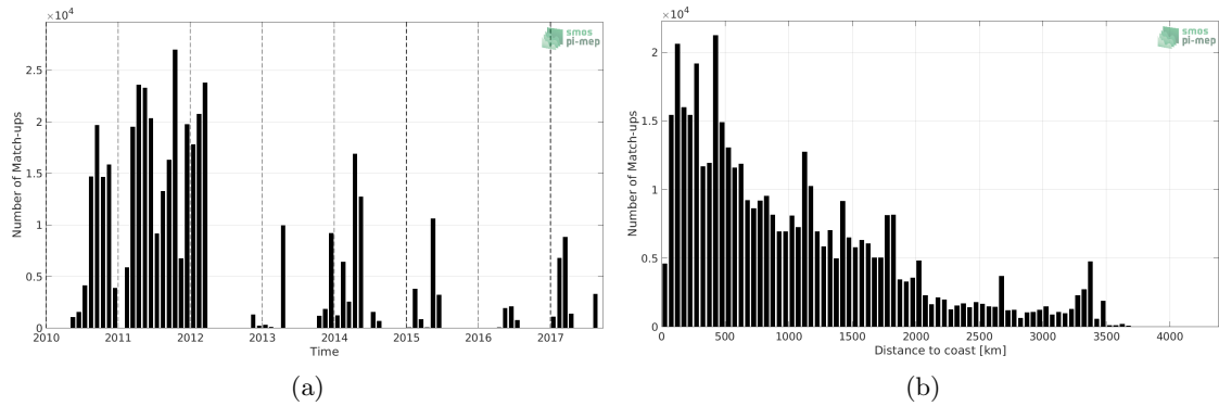
Figure 1: Number of match-ups between TSG (GOSUD-Sailing-ship) and SMOS L4 v2 Weekly (CATDS-CECOS-IFREMER) SSS as a function of time (a) and as function of the distance to coast (b) over the Mid-Low Latitudes 45N-45S Pi-MEP region and for the full satellite product period.
