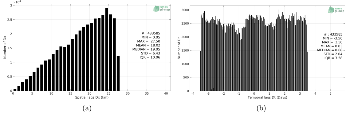
Figure 5: Histograms of the spatial (a) and temporal (b) lags between the location/time of the TSG (GOSUD-Sailing-ship) measurement and the date of the corresponding SMOS L4 v2 Weekly (CATDS-CECOS-IFREMER) SSS pixel.
