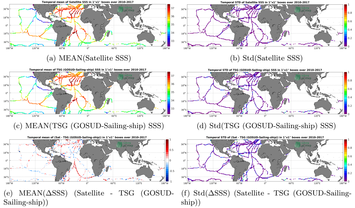
Figure 6: Temporal mean (left) and Std (right) of SSS from SMOS L4 v2 Weekly (CATDS-CECOS-IFREMER) (top), TSG (GOSUD-Sailing-ship) (middle), and of \Delta SSS (Satellite - TSG (GOSUD-Sailing-ship)). Only match-up pairs are used to generate these maps.
