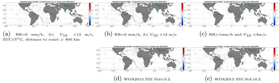
Figure 12: Temporal mean gridded over spatial boxes of size 1^\circ \times 1^\circ of \Delta SSS (SMOS L4 v2 Weekly (CATDS-CECOS-IFREMER) - TSG (GOSUD-Sailing-ship)) for 5 different subdatasets corresponding to: RR=0 mm/h, 3 < U_{10} < 12 m/s, SST > 5^\circ C , distance to coast > 800 km (a), RR=0 mm/h, 3 < U_{10} < 12 m/s (b), RR > 1 mm/h and U_{10} < 4 m/s (c), WOA2013 SSS Std < 0.2 (d), WOA2013 SSS Std > 0.2 (e).
