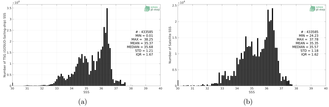
Figure 2: Histograms of SSS from TSG (GOSUD-Sailing-ship) (a) and SMOS L4 v2 Weekly (CATDS-CECOS-IFREMER) (b) considering all match-up pairs per bins of 0.1 over the Mid-Low Latitudes 45N-45S Pi-MEP region and for the full satellite product period.
