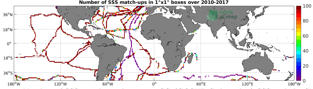
Figure 4: Number of SSS match-ups between TSG (GOSUD-Sailing-ship) SSS and the SMOS L4 v2 Weekly (CATDS-CECOS-IFREMER) SSS product for the Mid-Low Latitudes 45N-45S Pi-MEP region over 1°x1° boxes and for the full satellite product period.
