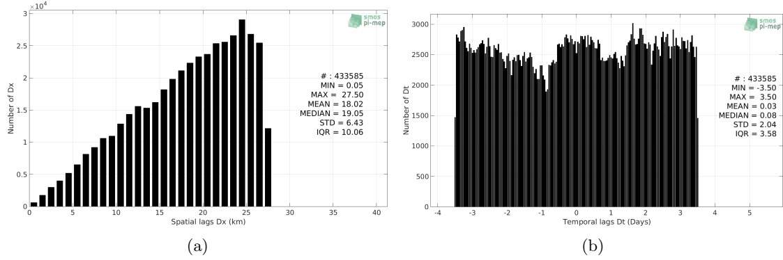
Figure 5: Histograms of the spatial (a) and temporal (b) lags between the time of the TSG-GOSUD-Sailing-ship measurements and the date of the corresponding SMOS-L4-CATDS-CECOS-IFREMER-V2-WEEKLY-0.5DEG SSS product.
