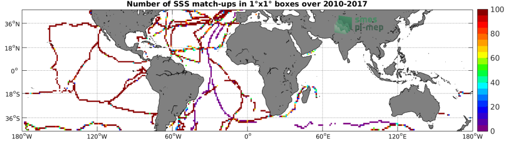
Figure 4: Number of SSS match-ups between TSG-GOSUD-Sailing-ship SSS and the SMOS-L4-CATDS-CECOS-IFREMER-V2-WEEKLY-0.5DEG SSS product for the Mid-Low Latitudes 45N-45S Pi-MEP region over 1°x1° boxes and for the full satellite product period.
