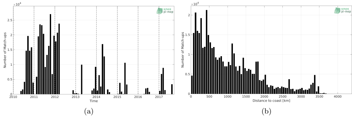
Figure 1: Number of match-ups between TSG-GOSUD-Sailing-ship and SMOS-L4-CATDS-CECOS-IFREMER-V2-WEEKLY-0.5DEG SSS as a function of time (a) and as function of the distance to coast (b) over the Mid-Low Latitudes 45N-45S Pi-MEP region and for the full satellite product period.
