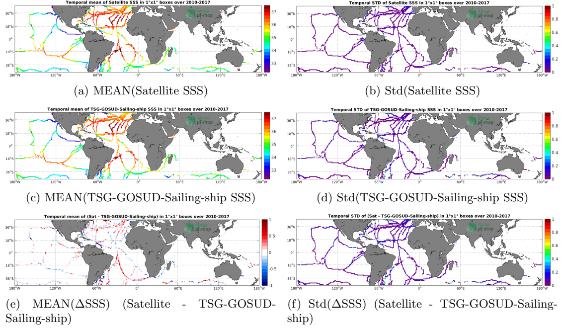
Figure 6: Temporal mean (left) and Std (right) of SSS from SMOS-L4-CATDS-CECOS-IFREMER-V2-WEEKLY-0.5DEG (top), TSG-GOSUD-Sailing-ship (middle), and of \Delta SSS (Satellite - TSG-GOSUD-Sailing-ship). Only match-up pairs are used to generate these maps.
