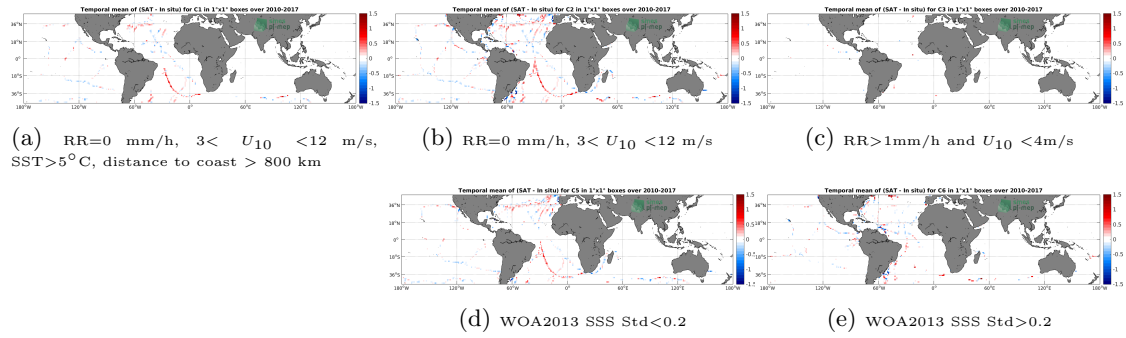
Figure 12: Temporal mean gridded over spatial boxes of size 1^\circ \times 1^\circ of \Delta SSS (SMOS-L4-CATDS-CECOS-IFREMER-V2-WEEKLY-0.5DEG - TSG-GOSUD-Sailing-ship) for 5 different subdatasets corresponding to: RR=0 mm/h, 3 < U_{10} < 12 m/s, SST > 5^\circ C , distance to coast > 800 km (a), RR=0 mm/h, 3 < U_{10} < 12 m/s (b), RR > 1 mm/h and U_{10} < 4 m/s (c), WOA2013 SSS Std < 0.2 (d), WOA2013 SSS Std > 0.2 (e).
