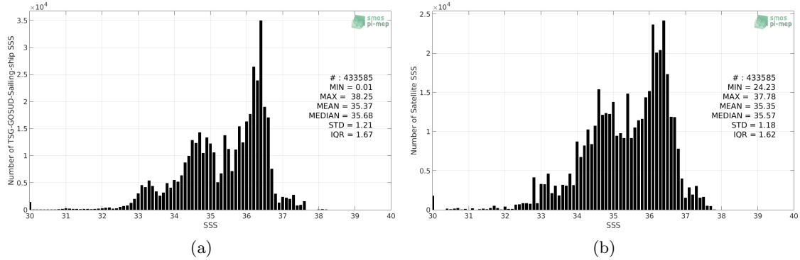
Figure 2: Histograms of SSS from TSG-GOSUD-Sailing-ship (a) and SMOS-L4-CATDS-CECOS-IFREMER-V2-WEEKLY-0.5DEG (b) considering all match-up pairs per bins of 0.1 over the Mid-Low Latitudes 45N-45S Pi-MEP region and for the full satellite product period.
