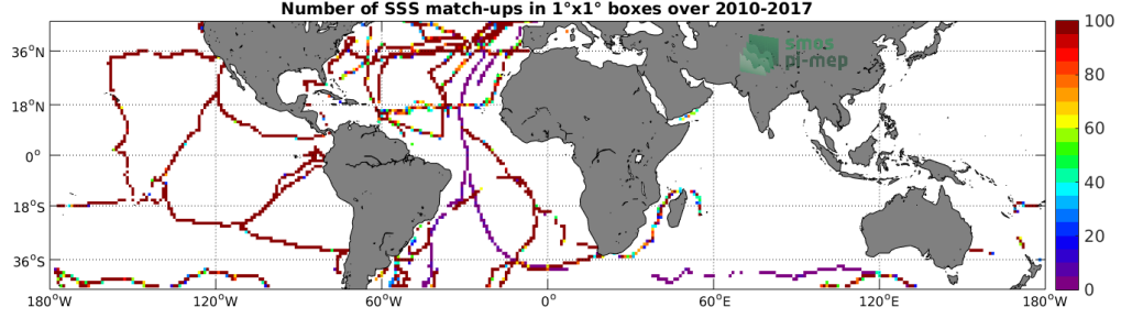
Figure 4: Number of SSS match-ups between TSG-GOSUD-Sailing-ship SSS and the SMOS-L4-CATDS-CECOS-IFREMER-V2-WEEKLY-0.5DEG SSS product for the Mid-Low Latitudes 45N-45S Pi-MEP region over 1^\circ \times 1^\circ boxes and for the full satellite product period.
