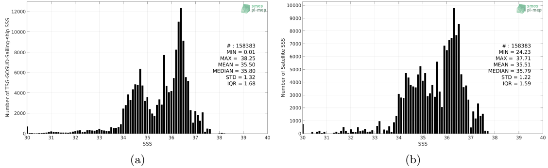
Figure 2: Histograms of SSS from TSG-GOSUD-Sailing-ship (a) and SMOS-L4-CATDS-CECOS-IFREMER-V2-WEEKLY-0.5DEG (b) considering all match-up pairs per bins of 0.1 over the Mid-Low Latitudes 45N-45S Pi-MEP region and for the full satellite product period.
