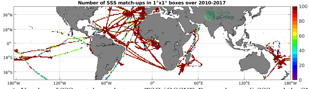
Figure 4: Number of SSS match-ups between TSG (GOSUD-Research-vessel) SSS and the SMOS L4 v2 Weekly (CATDS-CECOS-IFREMER) SSS product for the Mid-Low Latitudes 45N-45S Pi-MEP region over 1^\circ \times 1^\circ boxes and for the full satellite product period.
