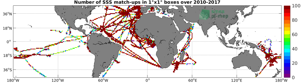
Figure 4: Number of SSS match-ups between TSG (GOSUD-Research-vessel) SSS and the SMOS L4 v2 Weekly (CATDS-CECOS-IFREMER) SSS product for the Mid-Low Latitudes 45N-45S Pi-MEP region over 1°x1° boxes and for the full satellite product period.
