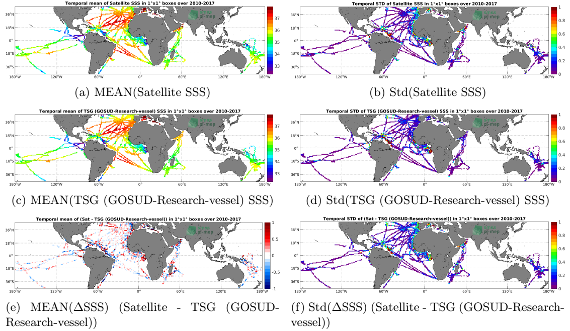
Figure 6: Temporal mean (left) and Std (right) of SSS from SMOS L4 v2 Weekly (CATDS-CECOS-IFREMER) (top), TSG (GOSUD-Research-vessel) (middle), and of \Delta SSS (Satellite - TSG (GOSUD-Research-vessel)). Only match-up pairs are used to generate these maps.
