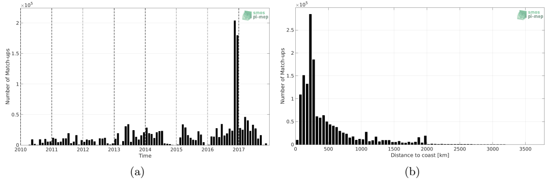
Figure 1: Number of match-ups between TSG (GOSUD-Research-vessel) and SMOS L4 v2 Weekly (CATDS-CECOS-IFREMER) SSS as a function of time (a) and as function of the distance to coast (b) over the Mid-Low Latitudes 45N-45S Pi-MEP region and for the full satellite product period.
