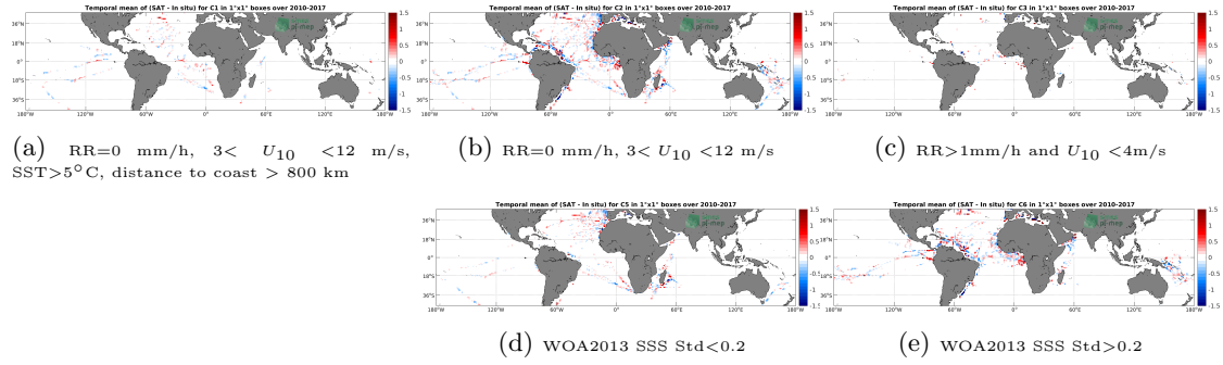
Figure 12: Temporal mean gridded over spatial boxes of size 1^\circ \times 1^\circ of \Delta SSS (SMOS L4 v2 Weekly (CATDS-CECOS-IFREMER) - TSG (GOSUD-Research-vessel)) for 5 different subdatasets corresponding to: RR=0 mm/h, 3 < U_{10} < 12 m/s, SST > 5^\circ C , distance to coast > 800 km (a), RR=0 mm/h, 3 < U_{10} < 12 m/s (b), RR > 1 mm/h and U_{10} < 4 m/s (c), WOA2013 SSS Std < 0.2 (d), WOA2013 SSS Std > 0.2 (e).
