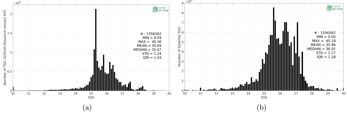
Figure 2: Histograms of SSS from TSG (GOSUD-Research-vessel) (a) and SMOS L4 v2 Weekly (CATDS-CECOS-IFREMER) (b) considering all match-up pairs per bins of 0.1 over the Mid-Low Latitudes 45N-45S Pi-MEP region and for the full satellite product period.
